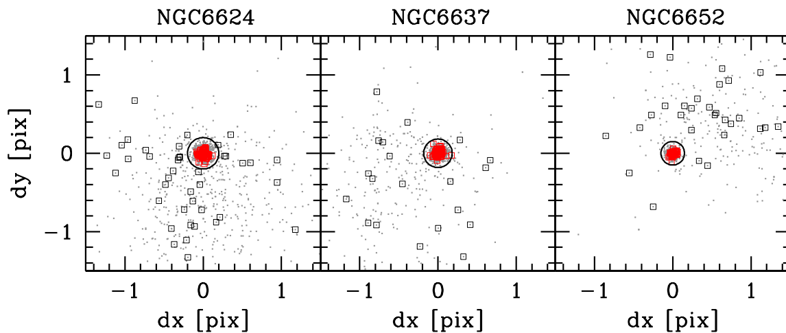
Fig. 1.— Vector-point diagrams (VPDs) for three clusters in the survey (see labels), showing the measured displacements (in ACS/WFC pixels) of stars brighter than the MS-TO level (with m_{F275W}^* < 0.5 ), over a \sim 7 -8 yr time-baseline. All stars within the circle (as well as stars with no displacement information) are assumed to be cluster members and have been included in the analysis, while those beyond the circle are considered as field contaminants. The red and black squares mark the cluster-member and the field-contaminant BSSs, respectively.
