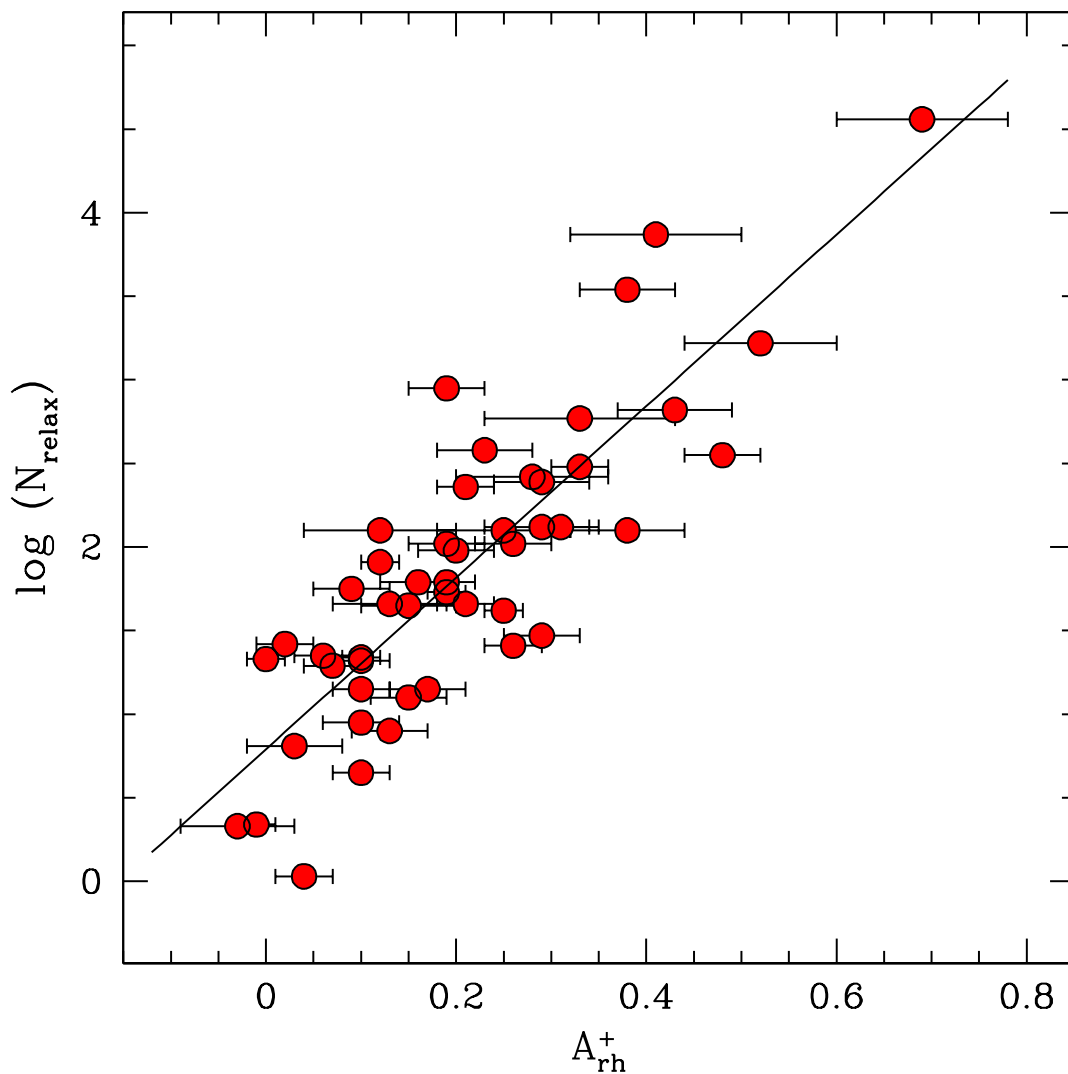
Fig. 9.— Relation between A_{rh}^+ and \log(N_{relax}) for the entire sample of 48 GCs. The parameter N_{relax} = t_{GC}/t_{rc} quantifies the number of current central relaxation times occurred since cluster formation. The tight relation between these two parameters demonstrates that the segregation level of BSSs measured by A^+ can be used to evaluate the level of dynamical evolution experienced by the parent cluster.
