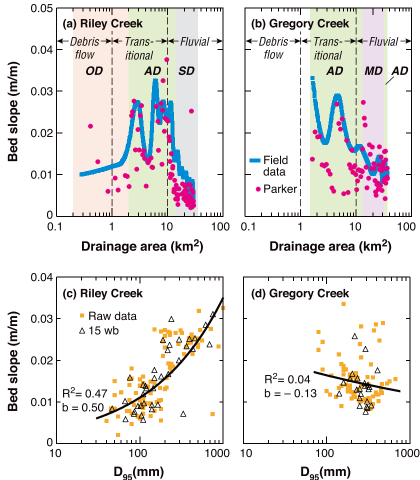
Figure 7. Plots showing the relation between channel slope (S), drainage basin area and D_{95} of Riley and Gregory creeks. The field data in panels (a) and (b) were smoothed using splines. Parker slope model is shown for comparison (panels (a) and (b)) and best fit line (panels (c) and (d)). b in panels (c) and (d) indicates the exponent of the best fit potential line (for the raw data). [Colour figure can be viewed at wileyonlinelibrary.com ]
