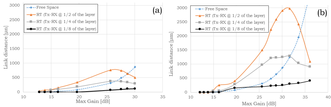
Figure 5. Link distance vs. antenna gain for different layer thicknesses: (a) 6 \mu\text{m} ; (b) 10 \mu\text{m} .
