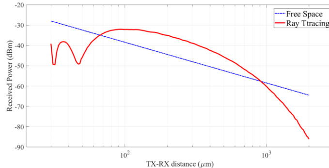
Figure 4. RT modeling of the in-layer propagation (layer thickness=4 \mu\text{m} , TX-RX middle placed, Vivaldi antennas at both the link ends)
