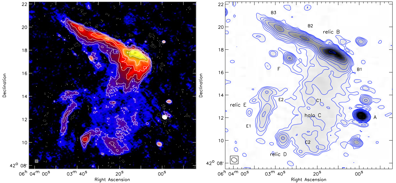
FIG. 1.— Left: LOFAR HBA 120–181 MHz image. The beam size is 8.0'' \times 6.5'' as indicated in the bottom left corner. Contour levels are drawn at [1, 2, 4, 8, \dots] \times 4\sigma_{\text{rms}} , with \sigma_{\text{rms}} = 93 \mu\text{Jy beam}^{-1} . Negative -3\sigma_{\text{rms}} contours are shown with dotted lines. Right: D-array VLA 1–2 GHz image with various sources labelled, following van Weeren et al. (2012a). Some of the sources are further subdivided into numbered components, e.g., relic E is divided into E1 and E2. The beam size is 31'' \times 24'' . Contour levels are drawn at the same levels as in the left panel, but with \sigma_{\text{rms}} = 35 \mu\text{Jy beam}^{-1} .
