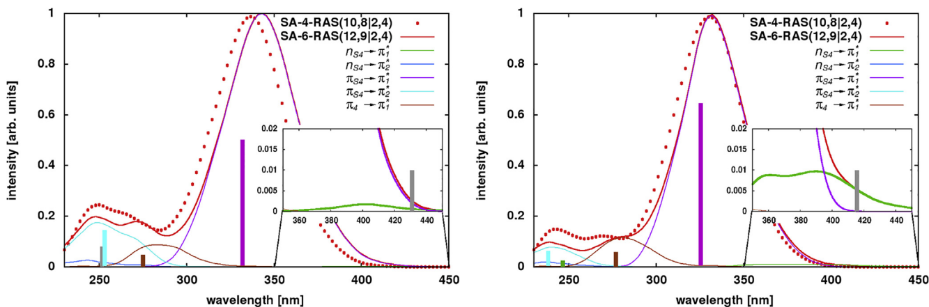
Fig. 6. State assignment in 4-thiouracil at the RASPT2/SA-6-RASSCF(12,9|2,4) level in the SS (left) and MS (right) flavors. Values at the equilibrium geometry (Table 1) are shown as stick spectra. (For interpretation of the references to colour in this figure legend, the reader is referred to the web version of this article.)
