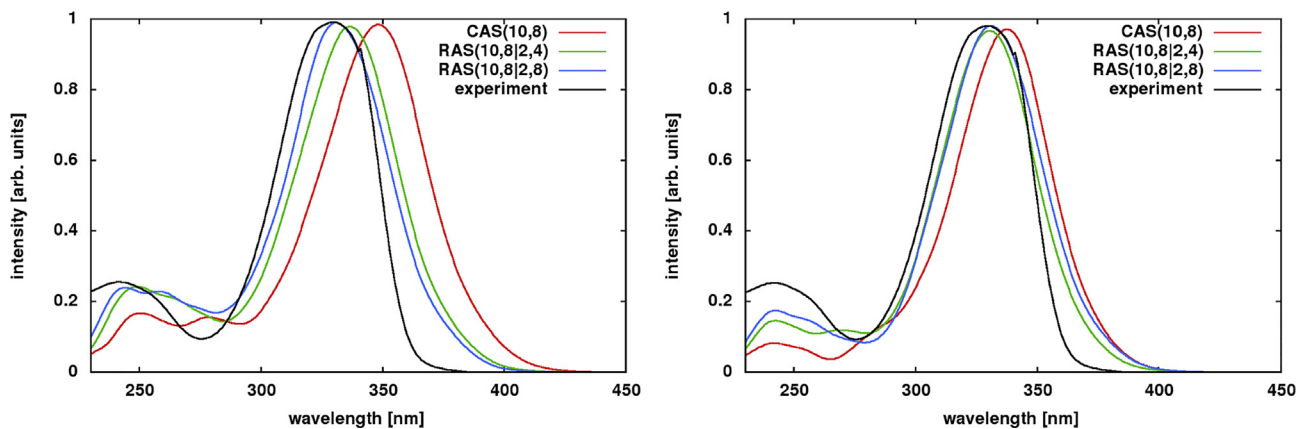
Fig. 5. Dependence of the LA spectrum of 4-thiouracil on the size of the active space size in the SS (left) and MS (right) flavors. Experimental spectrum in aqueous solution given as reference. (For interpretation of the references to colour in this figure legend, the reader is referred to the web version of this article.)
