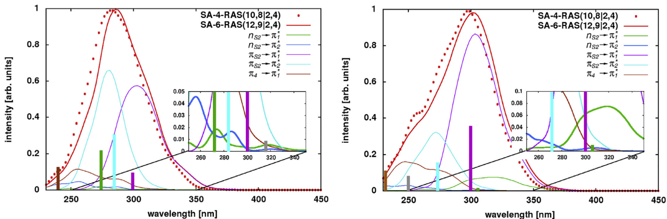
Fig. 3. State assignment in 2-thiouracil at the RASPT2/SA-6-RASSCF(12,9|2,4) level in the SS (left) and MS (right) flavors. Values at the equilibrium geometry (Table 1) are shown as stick spectra. (For interpretation of the references to colour in this figure legend, the reader is referred to the web version of this article.)
