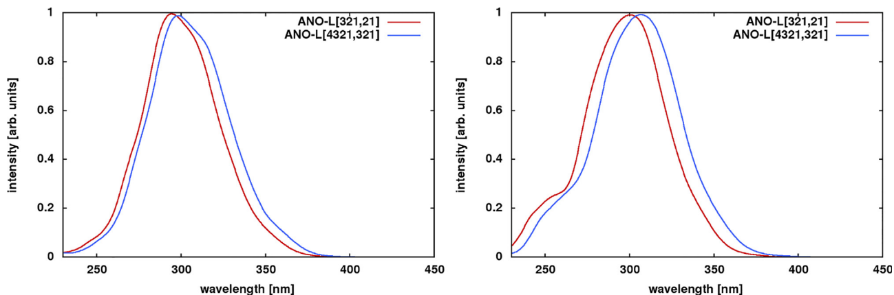
Fig. 4. Dependence of the LA spectrum of 2-thiouracil on the basis set size in the SS (left) and MS (right) flavors.
