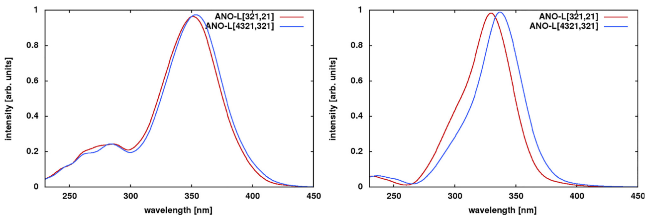
Fig. 7. Dependence of the LA spectrum of 4-thiouracil on the basis set size in the SS (left) and MS (right) flavors.
