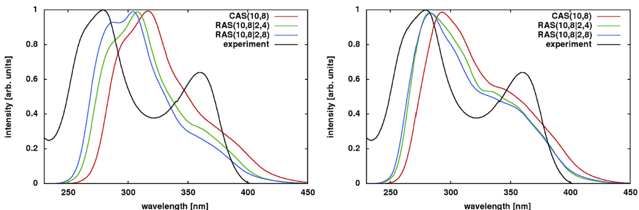
Fig. 8. Dependence of the LA spectrum of 2,4-thiouracil on the size of the active space size in the SS (left) and MS (right) flavors. Experimental spectrum in aqueous solution given as reference. (For interpretation of the references to colour in this figure legend, the reader is referred to the web version of this article.)
