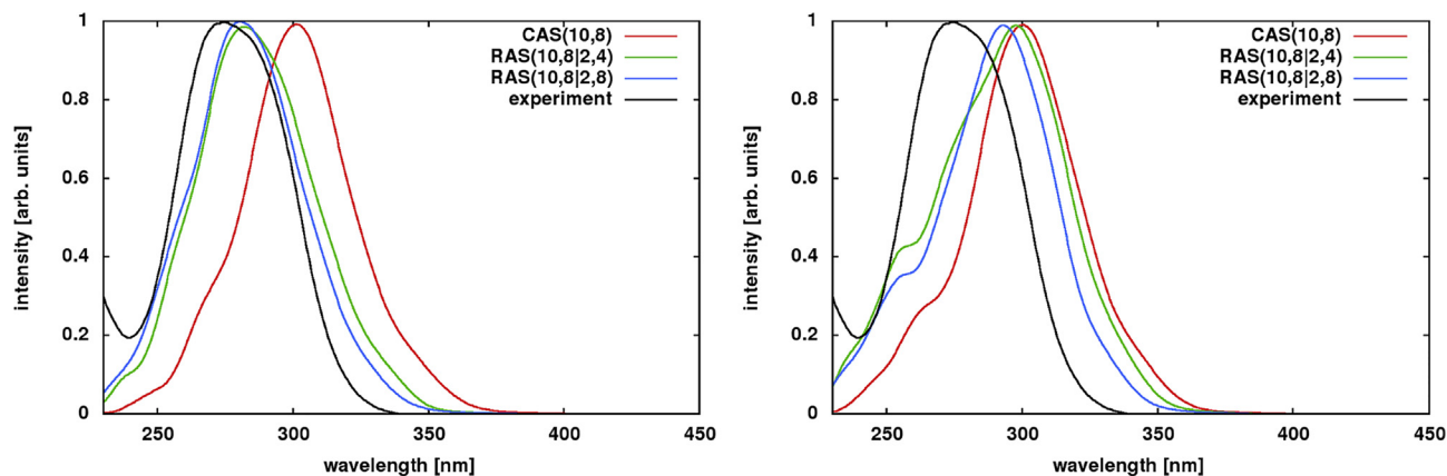
Fig. 2. Dependence of the LA spectrum of 2-thiouracil on the size of the active space size in the SS (left) and MS (right) flavors. Experimental spectrum in aqueous solution is given as reference. (For interpretation of the references to colour in this figure legend, the reader is referred to the web version of this article.)
