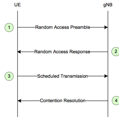
Fig. 7. Contention-based Random Access in NR.
