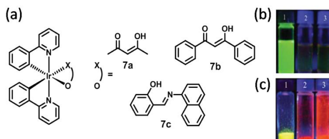
Figure 6: (a) Formula of cyclometallated Ir(III) complexes containing different ancillary ligands. Luminescence of 7a (1), 7b (2) and 7c (3) in \text{CH}_2\text{Cl}_2 solution (b) and solid state (c) ( \lambda_{\text{ex}} = 365 \text{ nm} ). Adapted from ref. [48] with permission from The Royal Society of Chemistry.
