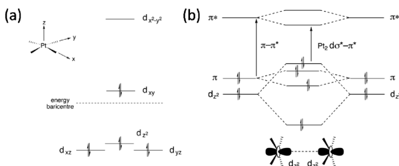
Figure 12: (a) Simplified orbital diagram of d orbitals for Pt(II) square planar complexes. (b) Simplified molecular orbital (MO) diagram of two interacting square-planar platinum(II) complexes, showing the intermolecular d z 2 orbital overlap in the ground-state and its influence on the energy of the MO levels. Adapted from ref. [70] with permission. Copyright © 2007, Springer-Verlag Berlin Heidelberg.
