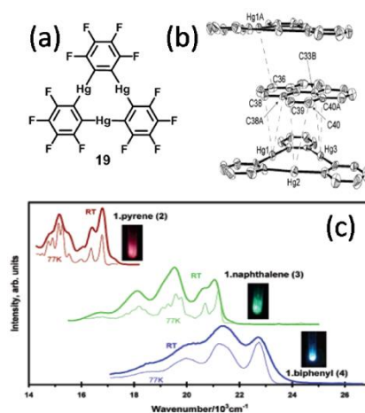
Figure 20: (a) Formula of a trinuclear Hg(II) complex. (b) Crystal structure of the columnar stacks formed by complex 19 and pyrene. (c) Phosphorescence spectra of the columnar stacks containing pyrene, naphthalene and biphenyl at 77K and room temperature (photos at RT under UV irradiation). Adapted with permission from ref. [98]. Copyright 2003 American Chemical Society.
