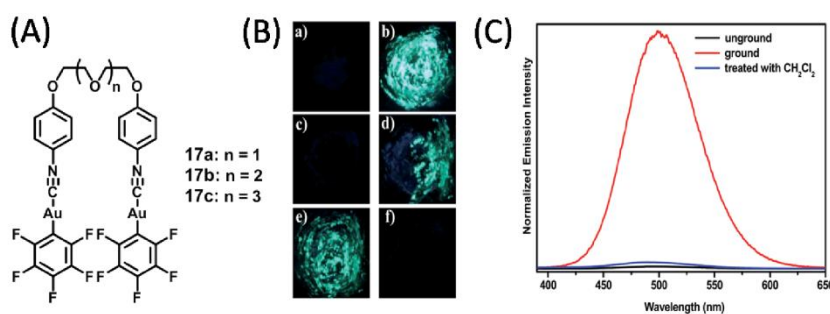
Figure 17: (A) Formulae of dinuclear Au(I) complexes. (B) Photographs of 17a under 365nm excitation: (a) before grinding, (b) after grinding, (c) after treatment with dichloromethane, (d) and (e) repetition of the green emission by grinding the powder with a pestle at room temperature, (f) annealing (at 100 °C for 30 s). (C) Emission spectra ( \lambda_{\text{exc}} = 350 \text{ nm} ) of 17a before grinding (black line), after grinding (red line), and after treatment with dichloromethane (blue line). Adapted from ref. [87] with permission from The Royal Society of Chemistry.
