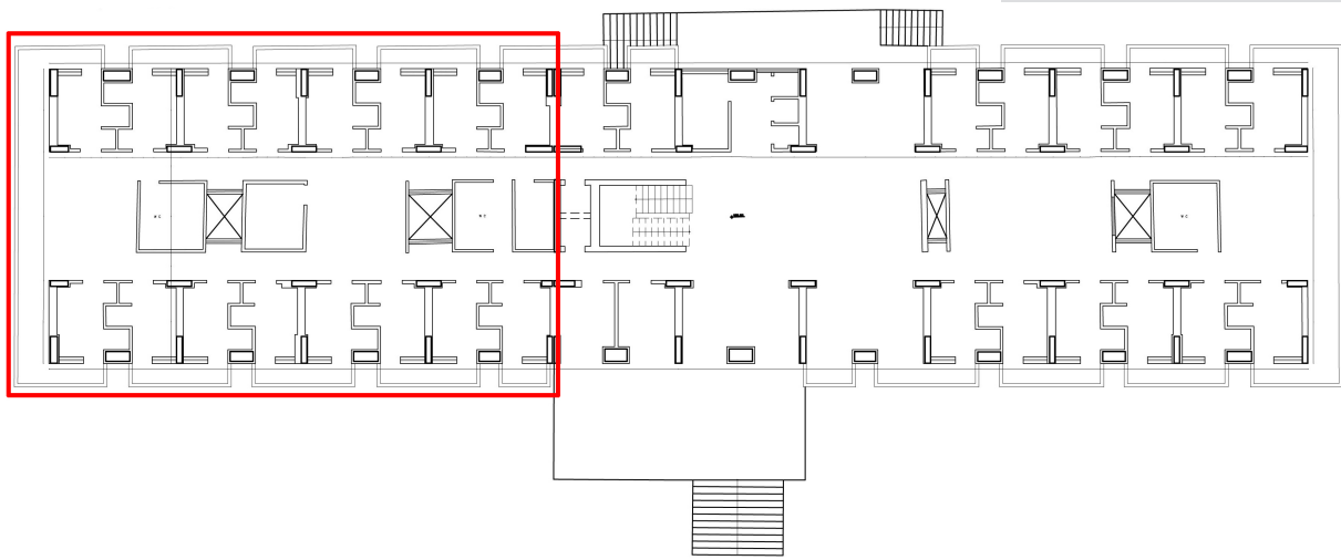
Figure 1. Architectural horizontal cross section of the Athens student house. The part of the structure subject to the improvement intervention is indicated.
