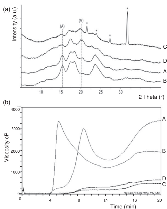
Figure 1 Crystallinity and viscosity in the mutant wheats and the control Cadenza. (a) X-ray diffraction patterns of starch synthesized by (A) cv Cadenza (B) Cad-GBSSI* (C) Cad-SSIIa* and (D) Cad-SBEIIa*. Peaks diagnostic for A- and V-type crystals are indicated. The intensity is given in arbitrary units (a. u.). The asterisks indicate the presence of impurities in the sample. (b) Viscosity profiles as measured by RVA (A) cv Cadenza, (B) Cad-GBSSI*, (C) Cad-SSIIa* and (D) Cad-SBEIIa*.
