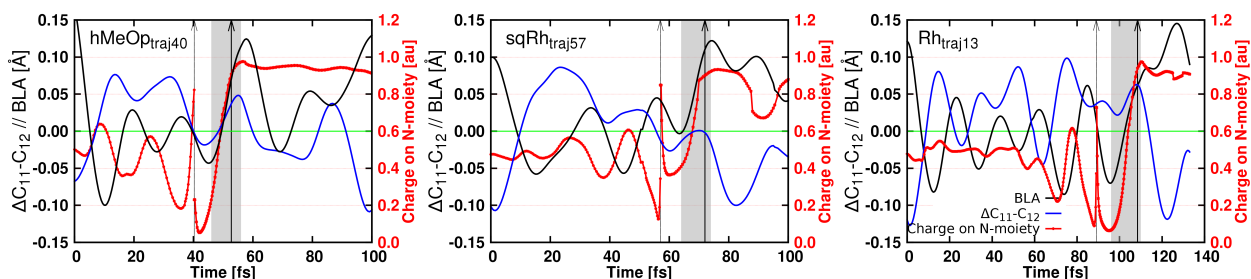
Figure 4. Selected examples show the evolution of BLA (bond-length alternation), C_{11}-C_{12} and charge on C_{11}-N fragment during the simulation in the three rhodopsins, ( \Delta C_{11}-C_{12} represents the deviation of C_{11}-C_{12} from 1.45\text{\AA} ), gray-shaded areas denote the time span in which the WF changes from CT to covalent after a hopping event, vertical dashed and solid arrows show the hopping and decision times, respectively.
