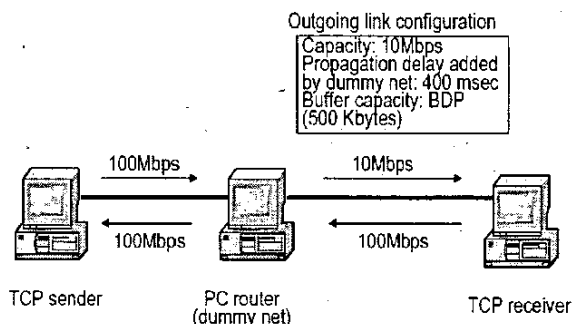
Figure 16. Measurement topology and configuration
