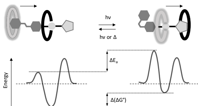
Figure 1. Schematic representation (top) and simplified potential energy curves (bottom) for the operation of an artificial molecular pump triggered by light.
