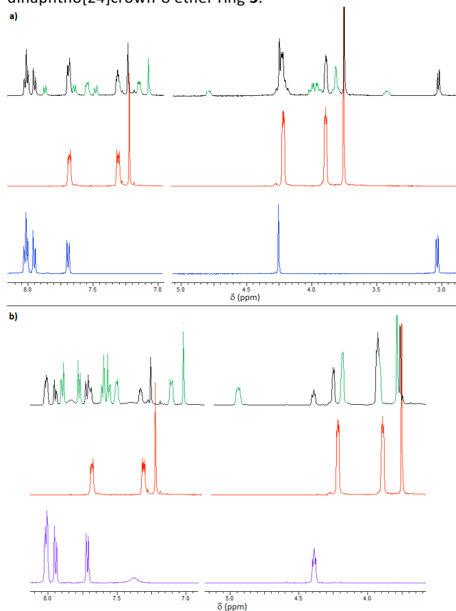
Figure 5. ^1\text{H} -NMR spectra (500 MHz, 298 K, \text{CD}_3\text{CN} ) of 3 mM solutions of free compounds and of an equimolar mixture of the components. a) Blue line: 1\text{H}^+ ; red line: 3 ; black line: 1:1 mixture solution, the peaks of the complex are highlighted in green. b) Purple line: 2\text{H}^+ ; red line: 3 ; black line: 1:1 mixture solution, the peaks of the complex are highlighted in green.
