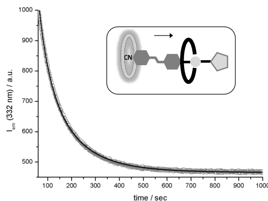
Figure 7. Emission changes at 332 nm observed as a function of time after mixing two equimolar solutions of 3 and 1H^+ ( 2.3 \times 10^{-6} M). The solid line is the fitting of the data with a mixed order model (see text for details). The cartoon is a schematic representation of the unidirectional threading process of crown 3 from the ( p -cyano)azobenzene extremity of 1H^+ .
