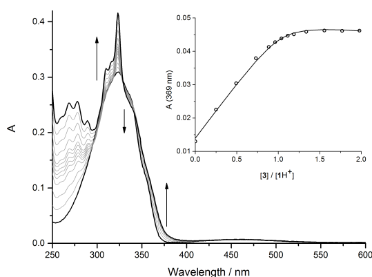
Figure 6. Absorption spectra of a 1.1 \times 10^{-6} M solution of 1H^+ upon titration with 3 . The inset shows the absorption changes at 369 nm (white circles) and the fitting of the data (solid line).
