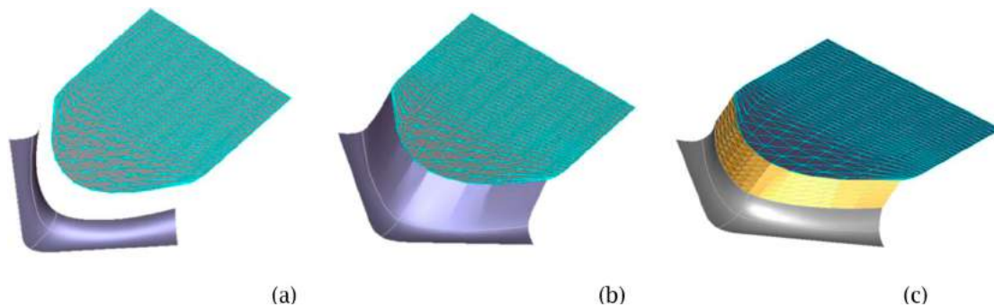
Figure 7. Example of 1-1 Face-Join: (a) Mesh-Face (top) and NURBS surface (bottom); (b) Case I, result of C^0 join; (c) Case II, result of AG^0 join.
