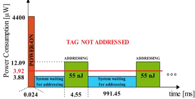
Fig. 5. Power and energy consumption of addressed tags at an activation rate of 1 Hz.
