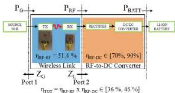
Figure 9. Schematic representation of a wireless battery charger.
