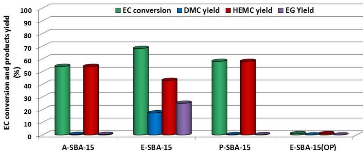
Figure 4 - Catalytic results: \text{CH}_3\text{OH}:\text{EC}=10:1 , T=65^\circ\text{C} , t=6 h, p = 1 bar, catalyst 5% w/w with respect to EC. EC conversion (green), DMC yield (blue), intermediate (HEMC) yield (red) and EG yield (violet).
