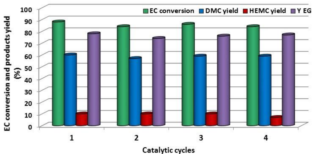
Figure 7 – Recycle tests of E-SBA-15. CH 3 OH:EC=10:1, T = 140°C, t=6 h, autoclave reactor purged with 10 bar of nitrogen, catalyst E-SBA-15, 5% w/w with respect to EC. EC conversion (green), DMC yield (blue), HEMC yield (red) and EG yield (violet).
