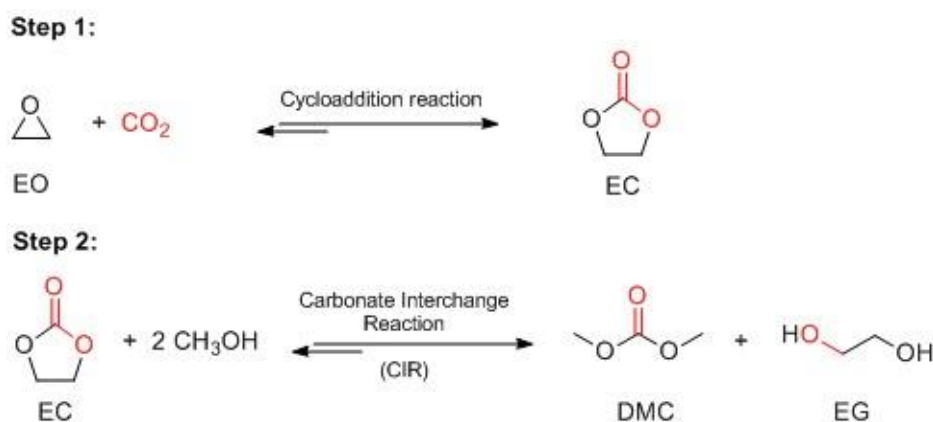
Scheme 1 - Two-step reaction for the synthesis of DMC.
