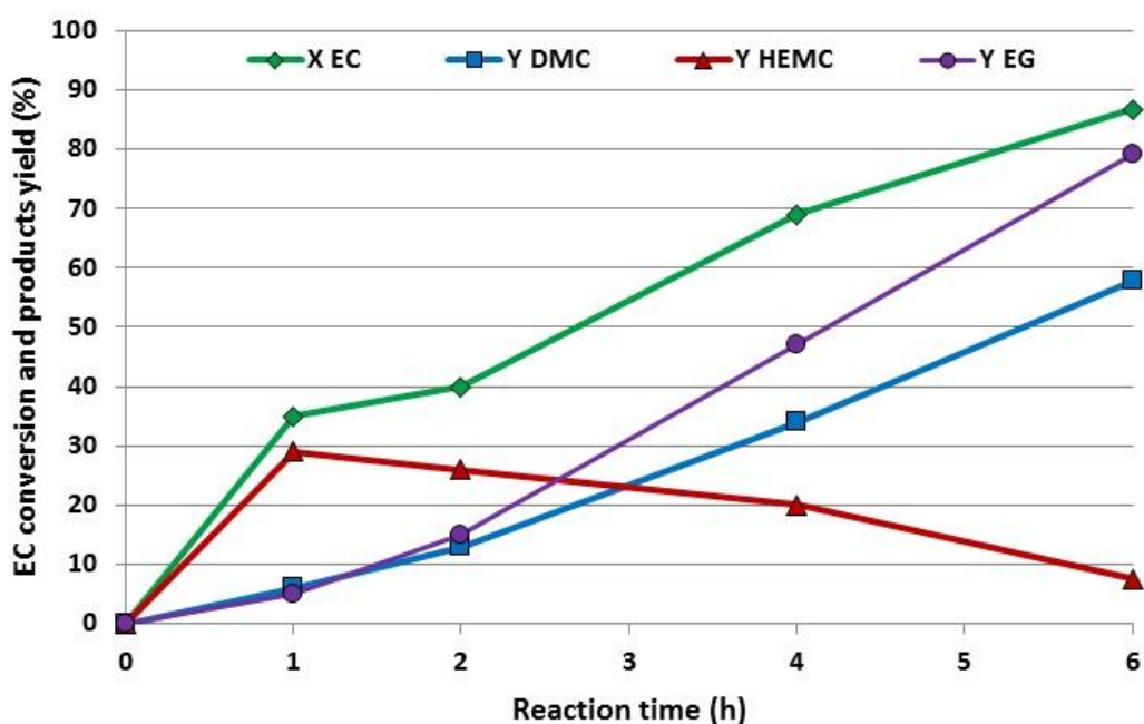
Figure 6 – Catalytic results as a function of the reaction time. \text{CH}_3\text{OH}:\text{EC}=10:1 , T = 140^\circ\text{C} , t=6 h, autoclave reactor purged with 10 bars of nitrogen, catalyst E-SBA-15, 5% w/w with respect to EC. EC conversion (green), DMC yield (blue), intermediate (HEMC) yield (red) and EG yield (violet).
