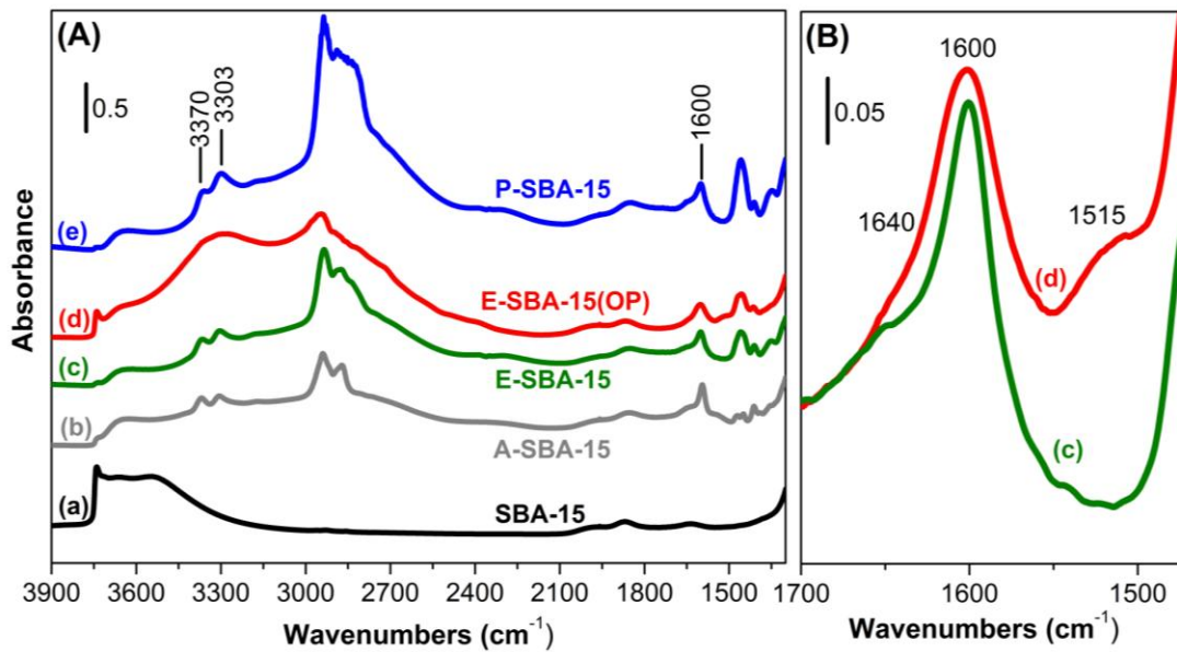
Figure 2 – Section (A): absorbance FT-IR spectra of plain SBA-15 (a, black) and of amino-modified A-SBA-15 (b, grey), E-SBA-15 (c, green), E-SBA-15(OP) (d, red) and P-SBA-15 (e, blue) samples after activation in vacuum at 150°C for 2 hours. Section (B) Magnification of the 1700-1470 \text{cm}^{-1} spectral range for E-SBA-15 (c, green) and E-SBA-15(OP) (d, red) samples.
