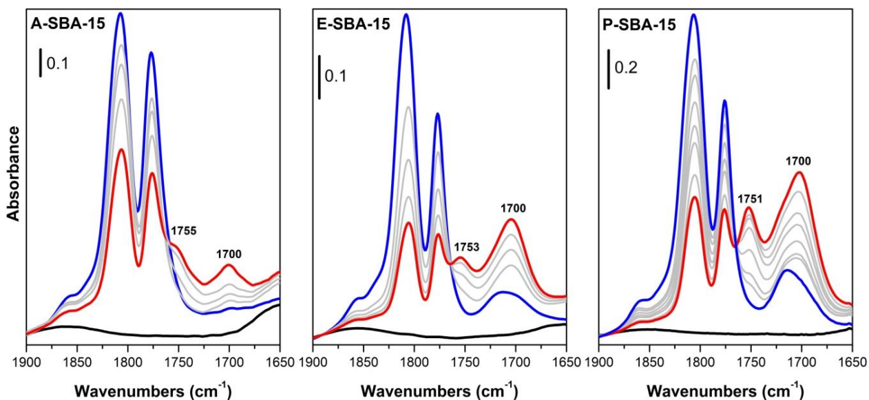
Figure 10 - Absorbance FT-IR spectra at BT, in the 1900\text{-}1650\text{ cm}^{-1} spectral range, after activation in vacuo at 150^\circ\text{C} (black spectrum), contact with ethylene carbonate (blue spectrum), and admission of 40 mbar of methanol: spectra recorded in time (light grey lines) up to 1 hour of contact (red spectra).
