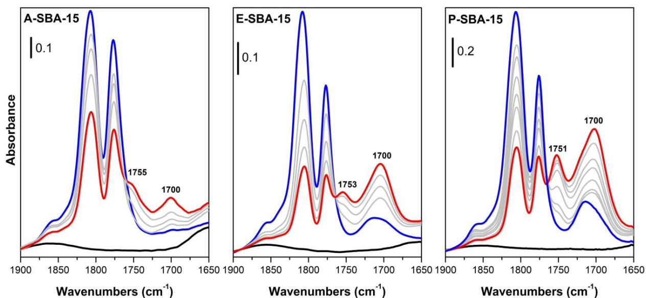
Figure 10 - Absorbance FT-IR spectra at BT, in the 1900\text{-}1650\text{ cm}^{-1} spectral range, after activation in vacuo at 150^\circ\text{C} (black spectrum), contact with ethylene carbonate (blue spectrum), and admission of 40 mbar of methanol: spectra recorded in time (light grey lines) up to 1 hour of contact (red spectra).
