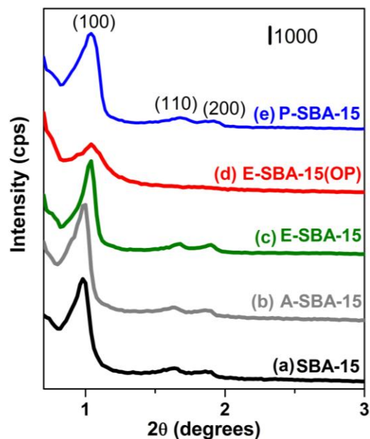
Figure 1- Low-angle XRD patterns of pure SBA-15 (a, black) and of amino-modified A-SBA-15 (b, grey), E-SBA-15 (c, green), E-SBA-15(OP) (d, red) and P-SBA-15 (e, blue) samples.
