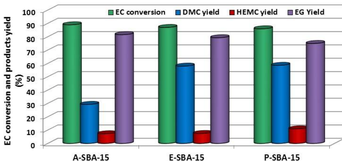
Figure 8 - Catalytic results, CH 3 OH:EC=10:1, T=140°C, t=6 h, autoclave reactor purged with 10 bars of nitrogen, catalyst 5% w/w on the respect of EC. EC conversion (green), DMC yield (blue), HEMC yield (red) and EG yield (violet).
