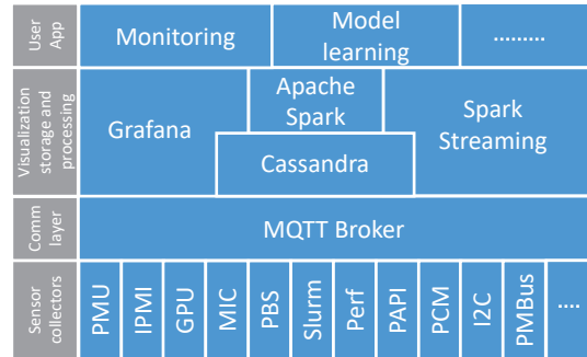
Fig. 1. Model-learning framework
