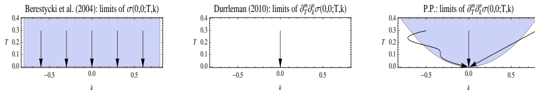
Fig. 1.1 Directions along which the limits are computed in Berestycki et al. (2004), in Durrleman (2010) and in this paper, respectively.
