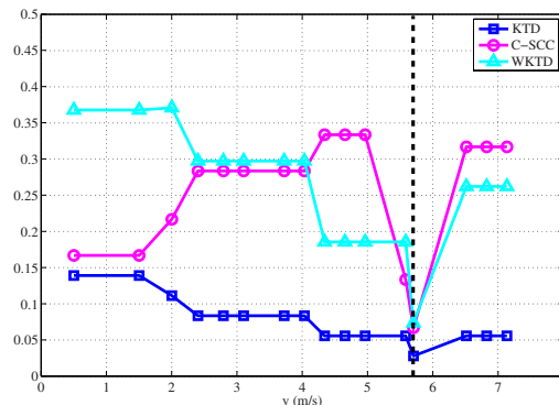
Fig. 4: Distances (KTD, C-SCC, and WKTD) between CRDS and the subjective tests, as a function of the parameter \bar{v} in (6), for the recorded scene.
