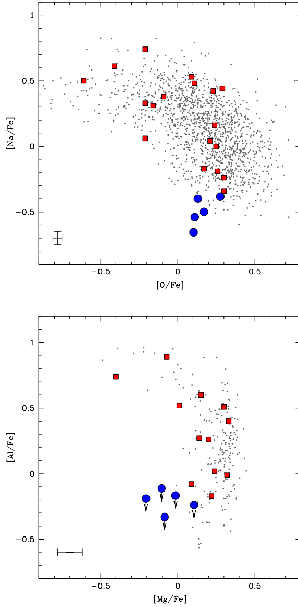
Fig. 6.— [O/Fe]-[Na/Fe] (top panel) and [Mg/Fe]-[Al/Fe] (bottom panel) diagrams. The blue solid circles are the target stars in NGC 121. For Al only upper limits have been derived. Red symbols mark stars in old LMC GCs from Mucciarelli et al. (2009a). Gray dots mark the values for stars in Galactic GCs (Carretta et al. 2009a,b).
