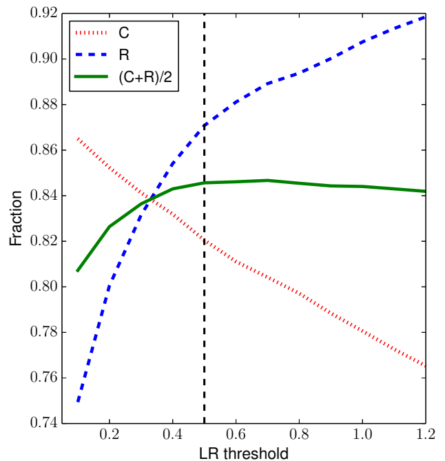
FIG. 1.— Completeness ( C , red dotted line), reliability ( R , blue dashed line) and (C+R)/2 (green solid line) at given values of L_{th} matching the optical catalog with new Legacy sources. The dashed black line shows the selected threshold in this band, L_{th}=0.5
