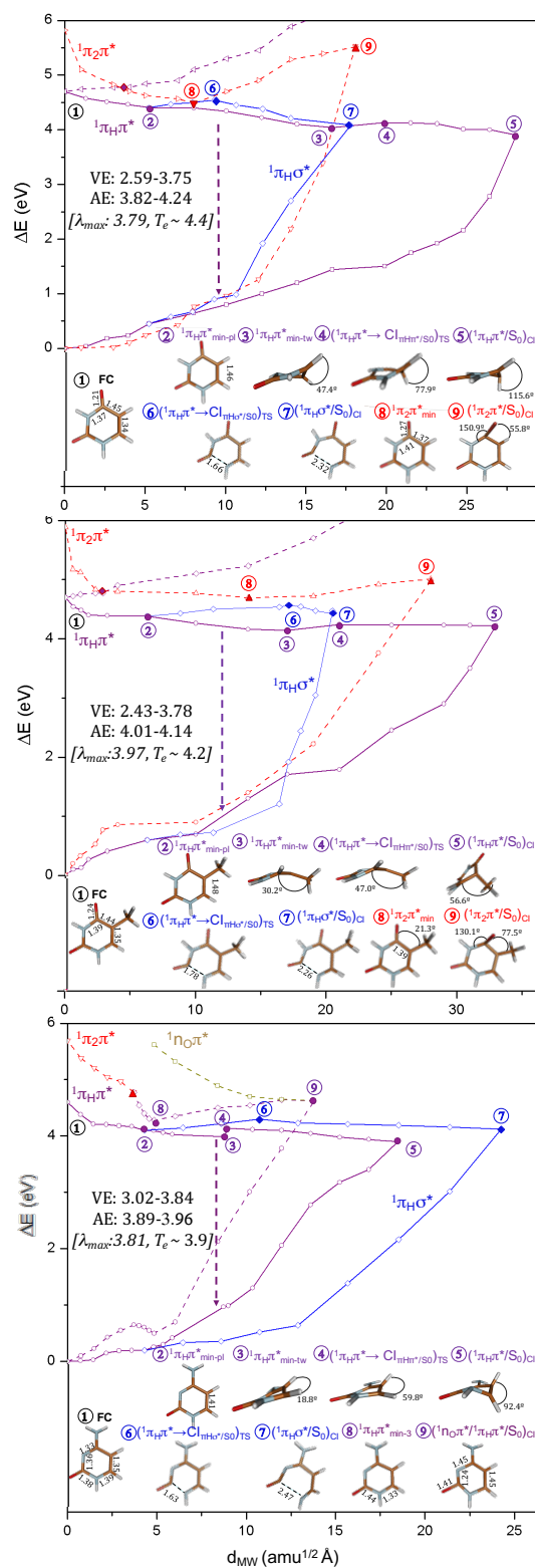
Figure 3. Evolution of the ground and lowest excited states for Urd (a), Thd (b) and Cyt (c) along the computed relaxation paths plotted in mass-weighted units. Full purple lines denote
