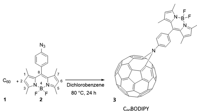
Scheme 1. Structures of the Analyzed Compounds
