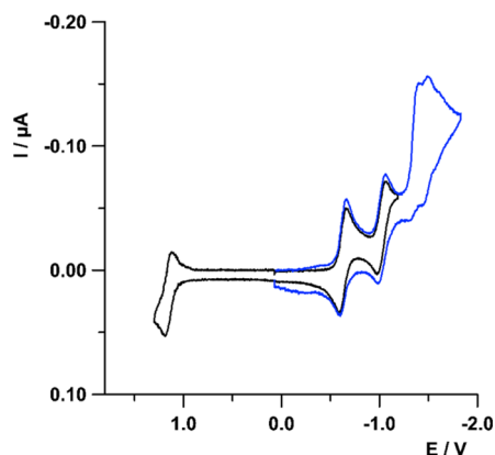
Figure 2. Cyclic voltammetric curves of species BODIPY- C_{60} 0.6 mM in 0.08 M TBAH/DCM solution. Sweep rate 1 V/s, working electrode Pt (125 \mu m, diameter), T = 25^\circ\text{C} .
