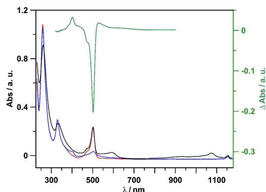
Figure 3. UV-vis-NIR spectra of the compound BODIPY- C_{60} 0.3 mM in 0.07 M TBAH/DCM solution; working electrode, Pt gauze; temperature = 0^\circ\text{C} . Spectra of the pristine compound (red trace), one-electron-oxidized species (blue trace), and one-electron reduced species (black trace). Difference spectrum of the oxidized state (green trace; pristine compound spectrum subtracted).
