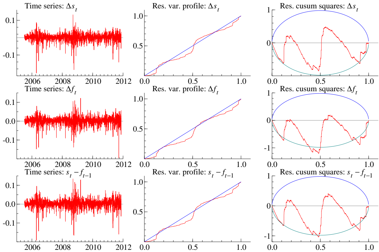
Figure 3. Graphics for silver
