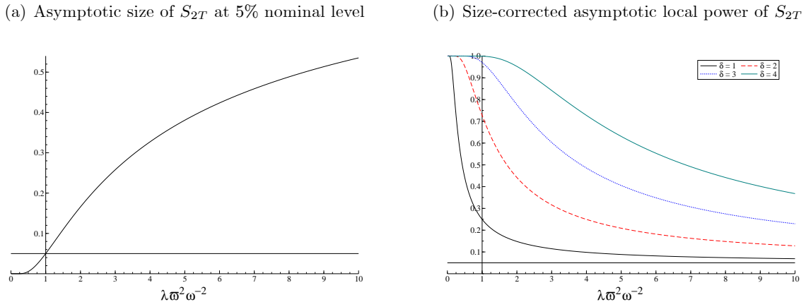
Figure 1. Size and power under heteroskedasticity
