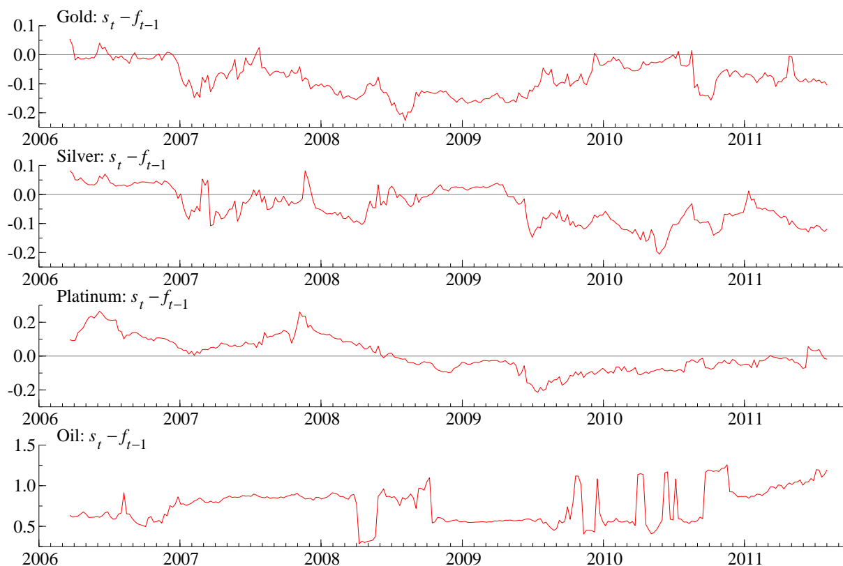
Figure 6. Rolling window estimates of d for spreads
