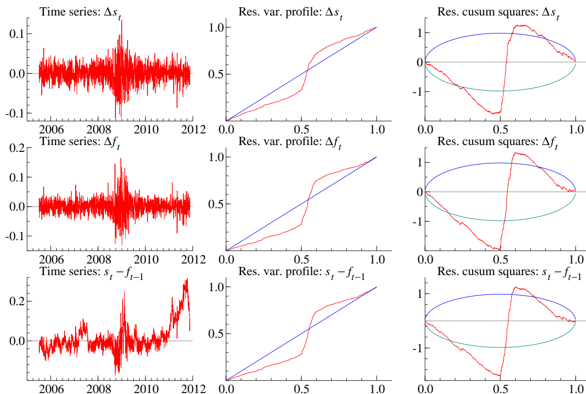
Figure 5. Graphics for crude oil
