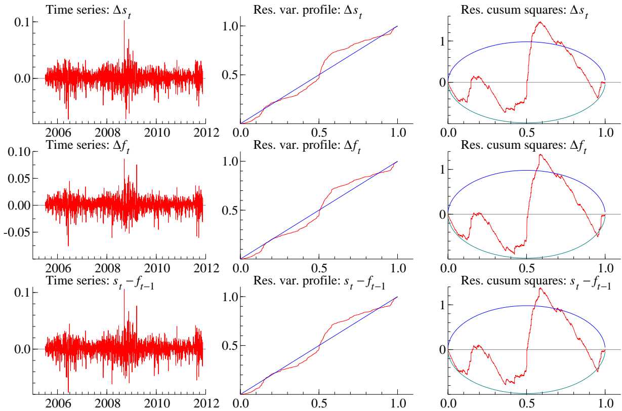
Figure 2. Graphics for gold
