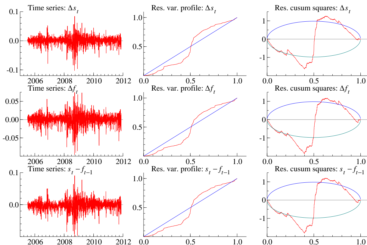
Figure 4. Graphics for platinum
