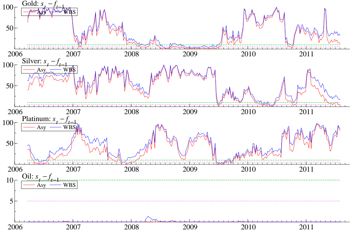
Figure 7. Rolling window tests of H_0 : d = 0 for spreads
