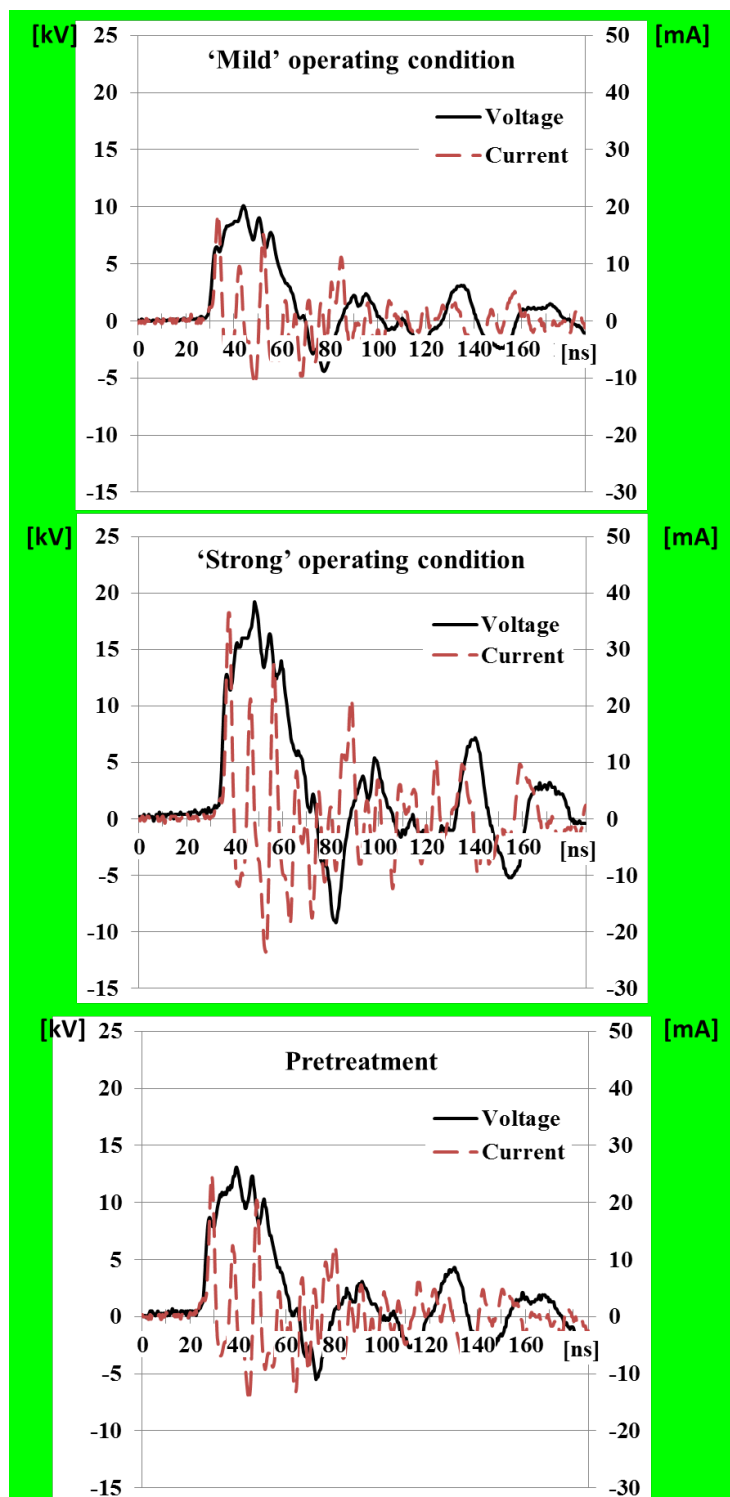
Figure S1. Recorded current and voltage waveform of the non-equilibrium atmospheric pressure nanopulsed plasma jet for the three operating conditions adopted during the tests: “mild” and “strong” plasma-polymerization and plasma pretreatment of the polymer substrate.
