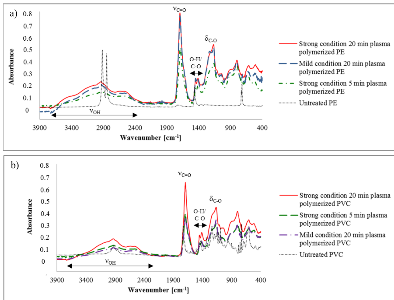
Figure 6. ATR-FTIR spectra of pristine PE and PE samples subjected to AA plasma polymerization process performed in “strong” operating condition: 5 and 20 min and in “mild” operating condition: 20 min (a); pristine PVC and PVC samples subjected to AA plasma polymerization process performed in “strong” operating condition: 5 and 20 min and in “mild” operating condition: 20 min (b).
