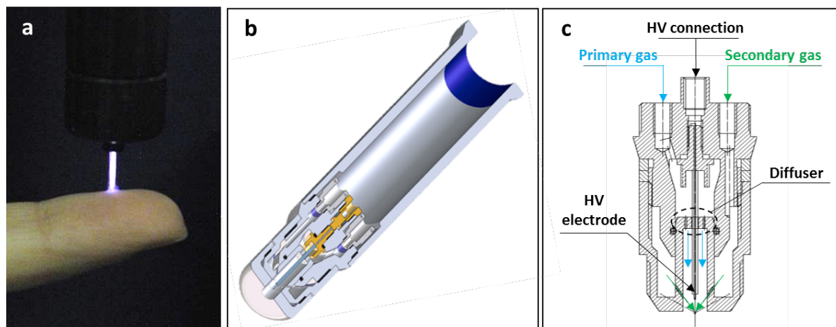
Figure 1. Non-equilibrium atmospheric pressure nanopulsed plasma jet: a) picture while impinging on biological substrate; b) assembly 3d rendering; c) schematic of the head of the plasma jet with gas diffuser and gas pathways highlighted.
