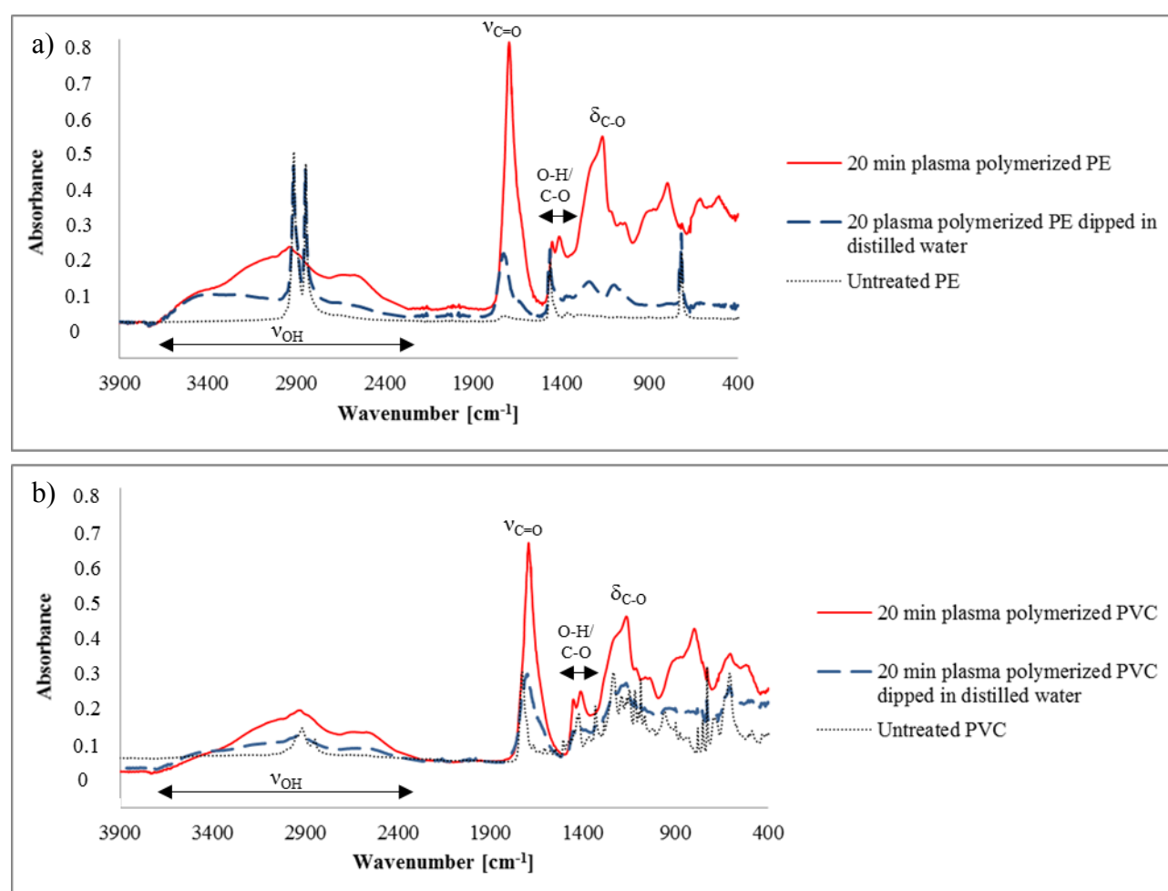
Figure 7. ATR-FTIR spectra of pristine PE and PE samples subjected to AA plasma polymerization process performed for 20 min in “strong” operating condition before and after being dipped in distilled water for 30 s (a); pristine PVC and PVC samples subjected to AA plasma polymerization process performed for 20 min in “strong” operating condition before and after being dipped in distilled water for 30 s (b).
