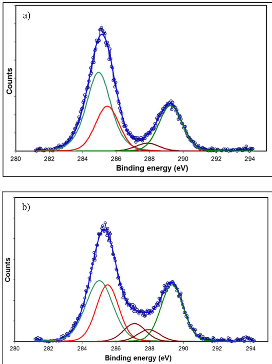
Figure 8. XPS deconvoluted C_{1s} peak of pPAA deposited on PE substrate by means of AA plasma polymerization process performed for 20 min in “mild” operating condition (a) and in “strong” operating condition (b).
