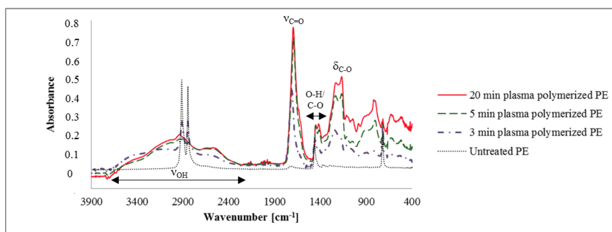
Figure 3. ATR-FTIR spectra of pristine PE and of PE substrates subjected to AA plasma polymerization process performed in “mild” operating conditions: 3, 5 and 20 min.
