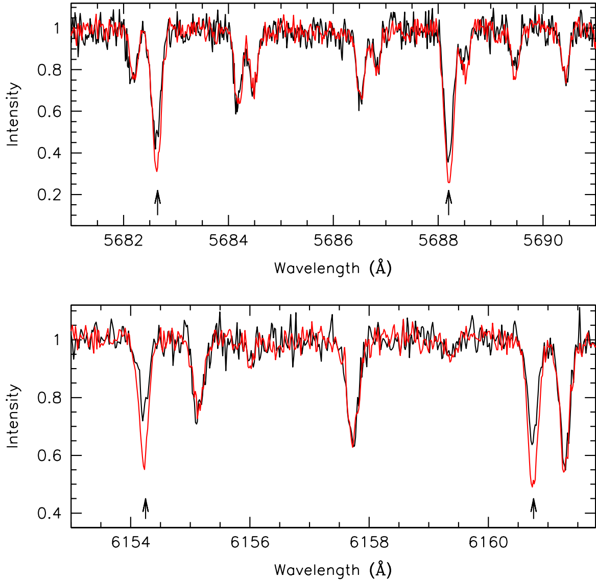
Fig. 8.— Comparison between the spectra of the RGB stars 89 (red line) and 95 (black line) for the NaI lines at 5682-5688 \text{\AA} (top-panel) and 6154-6160 \text{\AA} (bottom-panel). The black arrows mark the position of the Na lines.
