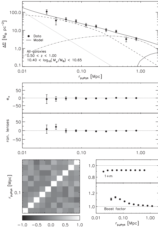
Figure C1. Galaxy–galaxy lensing measurements and systematic checks for the sample 10.40 < \log(M_*/M_\odot) < 10.65 . In the top panel, we show the data (dots with error bars) and the model (thick line) split into the stellar term in dotted line, the central term in dashed line, the satellite term in dot-dashed line and the two-halo term in black solid line at bottom-right corner. The lower panels show the systematic tests (rotated-shape signal and random lens positions), calibration factor (multiplicative bias correction and boost factor) and the lower-left corner the correlation coefficients of the correlation matrix from the jackknife estimate.
