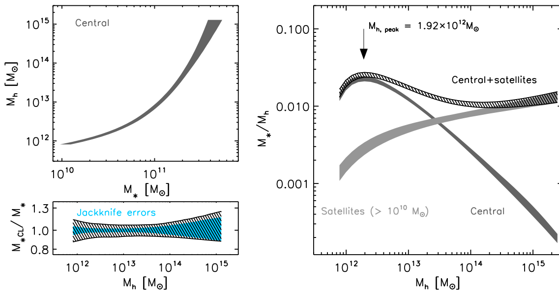
Figure 9. Best-fitting M_*-M_h relationship (left) and SHMR (right). The black shaded areas represent the confidence limits from the total errors. The bottom-left panel shows the confidence limits interval as a function of halo mass in the case of statistical errors (from jackknife resampling in light blue) and total errors (in black). The SHMR is derived as function of host halo mass for the central galaxy (dark grey), the satellites (light grey) and the sum of both (black). The peak value of the central SHMR is indicated by the black arrow.
