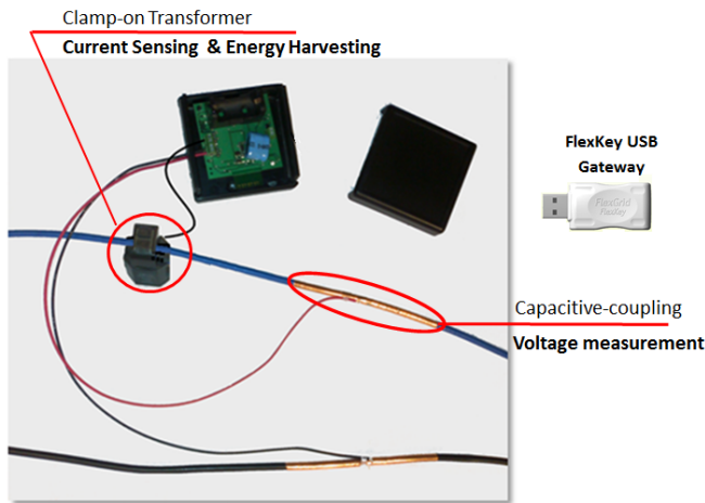
Fig. 4. Contact-less Smart power meter prototype.
