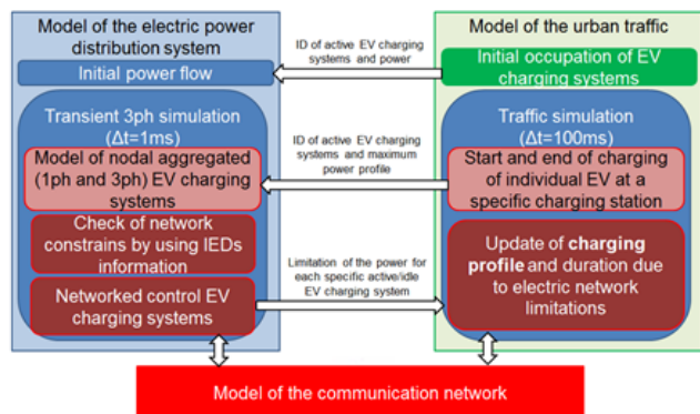
FIGURE 6. Data synchronization and exchange between traffic and power network simulators, communication simulator and power distribution simulator.
