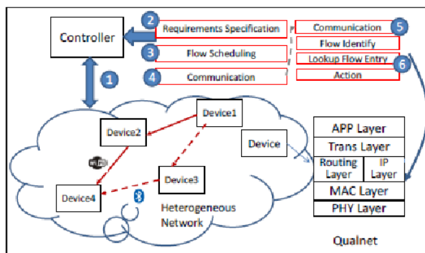
FIGURE 24. Operational flow diagram.
