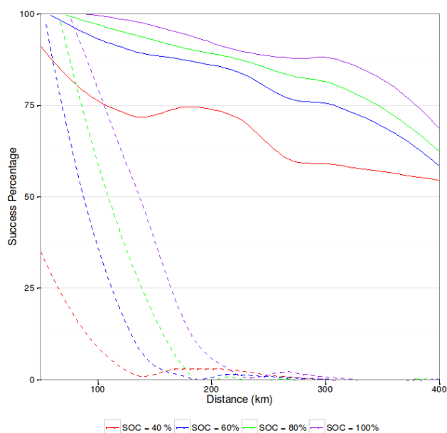
FIGURE 21. Success probability for the route planning service.
