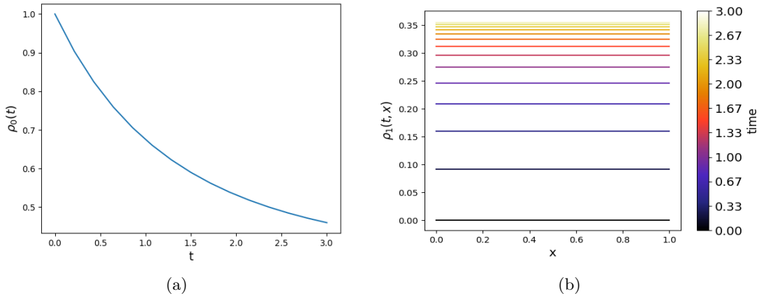
Figure 1: Solutions plots of the bCDME generated with constant creation and degradation rates with \lambda_c = \lambda_d = 0.5 . a. The solution of \rho_0(t) as a function of time. b. The solution of \rho_1(t, x_1) as a function of position and time.
