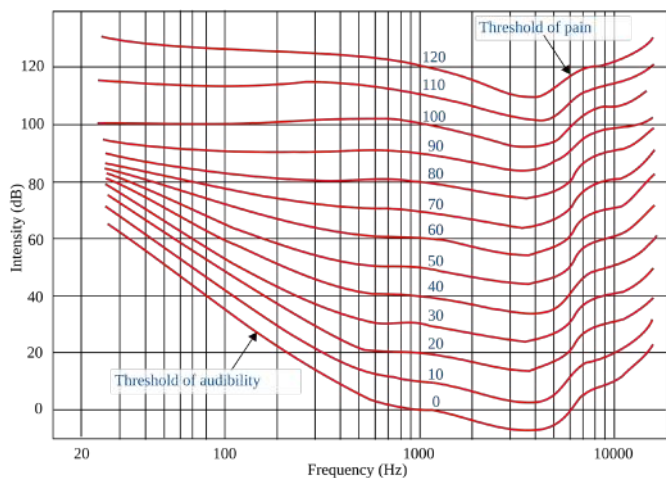
Fig. 4 – Fletcher-Munson equal loudness contours with threshold of audibility, threshold of pain, phons labels.
