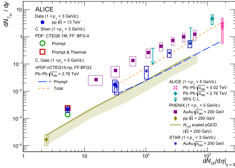
Fig. 4. Direct photon yield at midrapidity as a function of charged-particle multiplicity dN_{\text{ch}}/d\eta . The results from this letter are shown as two blue markers that correspond to the measurements in INEL and HM pp collisions at \sqrt{s} = 13 TeV, with the corresponding dN_{\text{ch}}/d\eta values taken from Ref. [59]. The results in INEL event class are compared to theoretical calculations for prompt (open green circle) and prompt+thermal (open red square) yields [35]. The results from the STAR [36], PHENIX [91,92] and ALICE [9,10] collaborations are shown as full markers of various colours, and the band shows N_{\text{coll}} -based extrapolation of pQCD calculations for pp collisions at \sqrt{s} = 200 GeV [93]. The Pb-Pb results are compared with the theoretical prediction by Gale [94], which includes prompt, pre-equilibrium and thermal photons. The prompt-photon yield is computed with NLO pQCD using the INCNLO code [95] together with the nCTEQ15 nuclear parton distribution function [96], and the BFG-II [84] fragmentation function.
