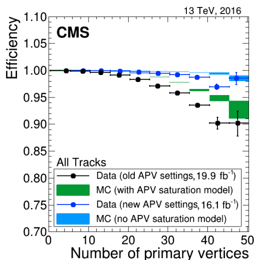
Figure 26. Tracking efficiency estimated using a tag-and-probe method as a function of the number of primary vertices for an inclusive muon track collection [36]. Data from early 2016 (black dots) and late 2016 (blue dots) are compared with two different MC simulations: one (blue) does not contain any special treatment of the APV25 preamplifier saturation, the second (green) contains a modeling of the preamplifier saturation to account for the reduced charge response of the amplifier under high-occupancy conditions.
