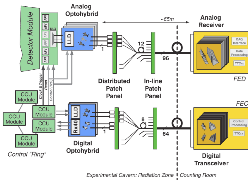
Figure 3. Overview of the control and readout scheme of the SST.
