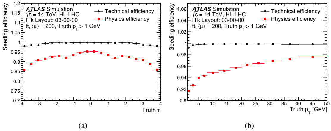
Figure 11. Expected technical and physics seeding efficiencies as a function of (a) \eta and (b) p_T for t\bar{t} events at \langle\mu\rangle = 200 for hard-scatter particles with p_T > 1 GeV. The efficiency is shown for the combined pixel and strip seeding.
