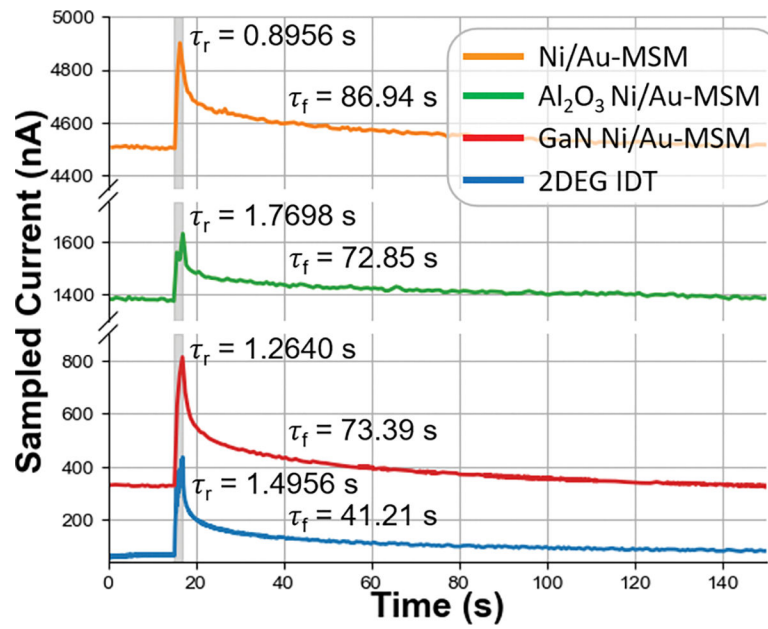
Fig. 3. Sampled current signals over time of the demonstrated Ni/Au-MSM, Al 2 O 3 Ni/Au-MSM, GaN Ni/Au-MSM, and 2DEG IDT detectors with annotated rise and fall times. Gray shaded regions indicate when the electron beam was on for a total dose of 129.6 Gy.
