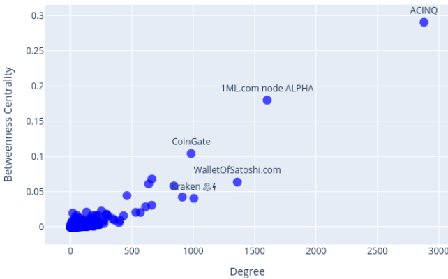
Fig. 2: Relationship between node degree and betweenness centrality on the 2025 snapshot.
