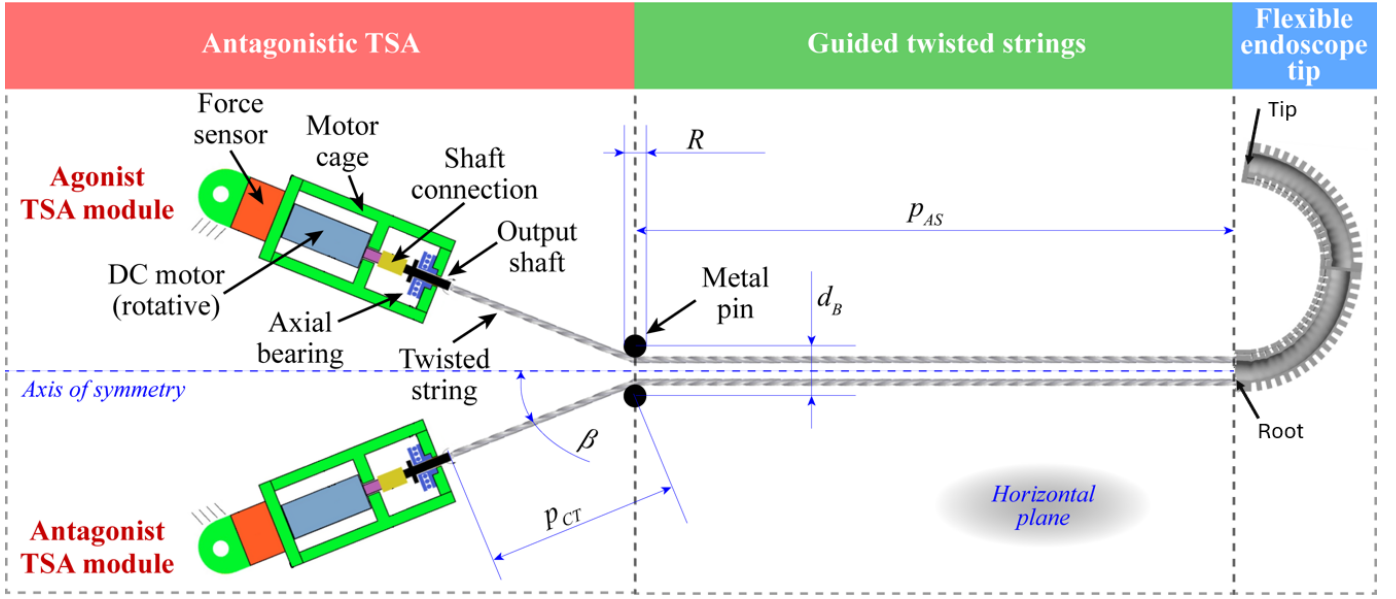
Fig. 1: Schematic representation of the antagonistically actuated flexible endoscope using two TSA modules (top view).
