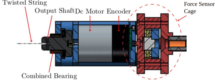
(a) Overall representation of the TSA module's components.
