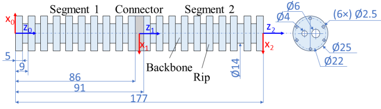
Fig. 2: The endoscope has two segments, each of which with a backbone with ribs. To accommodate the strings, ribs have six holes (unit measurement are mm). Two channels are present in the backbone for camera and instruments.
