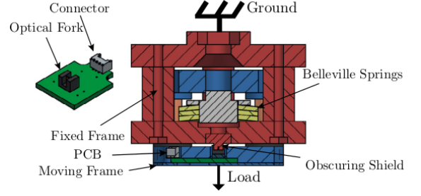
(b) Focus on the TSA module's force sensor.
