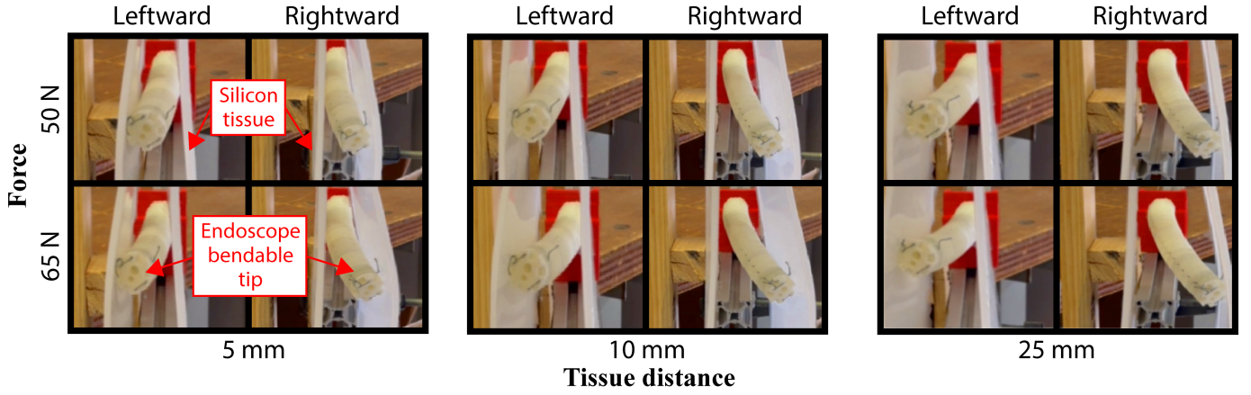
Fig. 6: Shots from the tissue interaction experimental validation, for the different combinations of reference force, tissue distance and endoscope tip bending direction.
