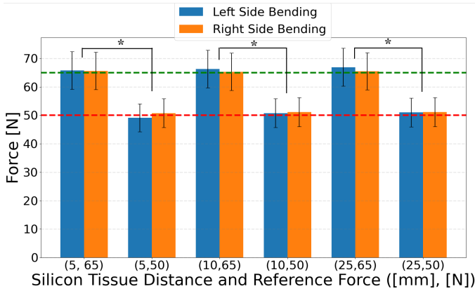
Fig. 7: Results of the tissue interaction experimental validation. Bars and whiskers indicate mean value and standard deviations, respectively. Symbol “*” indicates statistical significant difference, p < .05
