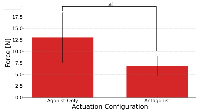
Fig. 8: Results of the stiffness increase experimental validation. Bars and whiskers indicate mean value and standard deviations, respectively. Symbol “*” indicates statistical significant difference, p < .05 .
