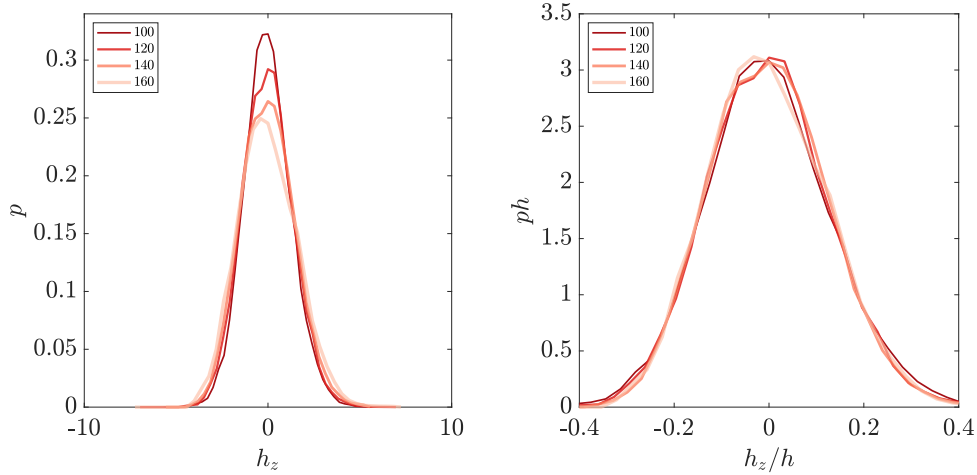
FIG. 3. TNTI probability density function (PDF) at t = [100, 120, 140, 160] in the left panel and the corresponding plots with the probability p against the distance h_z(x, y, t) of the TNTI from its average position normalised using the characteristic jet width h in the right panel.
