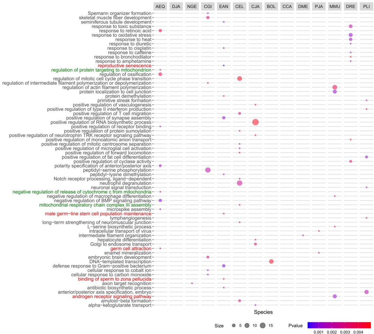
Fig. 5. GO enrichment analysis of biological processes performed on the supposed nuclear targets of smithRNAs, by species. Only GO supported by more than one gene are shown. See Fig. S3 for complete information and Fig. S4 for molecular functions and cellular components. Circle area represents the number of genes, the P -value is color coded. Go terms associated to mitochondrial and sex related functions are highlighted in green and red, respectively. See Table 1 for species abbreviations.
