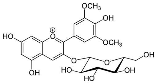
Malvidin-3-O-glucoside (Mv-3-O-glc)
