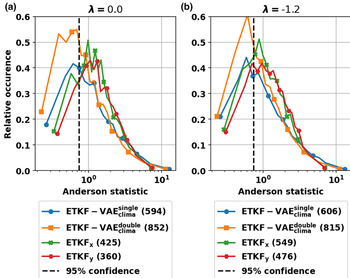
FIGURE 13 Left: probability distribution of the Anderson statistic for the different forecast ensembles of the latent variable in experiment ETKF\text{-}VAE^{\text{single}}_{\text{clima}} (blue), the latent variable in ETKF\text{-}VAE^{\text{double}}_{\text{clima}} (yellow), the x-coordinate in ETKF (green), and the y-coordinate in ETKF (red) in the case in which the observational error is not skewed. Right: same but now with the observational errors drawn from a skewed Gaussian distribution with skewness parameter \lambda = -1.2 . Also shown is the Anderson value above which the ensemble is different from Gaussian at 95% confidence and, between brackets, the number of times the Anderson metric of the ensemble is below this level.
