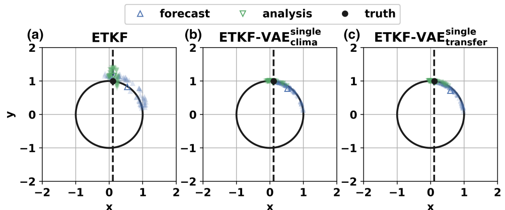
FIGURE 8 Truth (black), forecast ensemble (blue), and analysis ensemble at time 360 (green) for (a) ETKF , (b) ETKF-VAE single clima , and (c) ETKF-VAE single transfer . Ensemble means are depicted as triangles. The assimilated value of the x -coordinate is depicted as a dashed black line.
