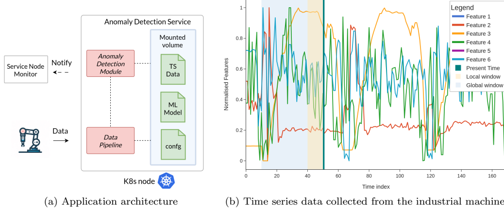
Figure 5: End-to-end anomaly-detection prototype: (a) Application architecture and (b) Example multivariate time-series collected from the industrial machines.
