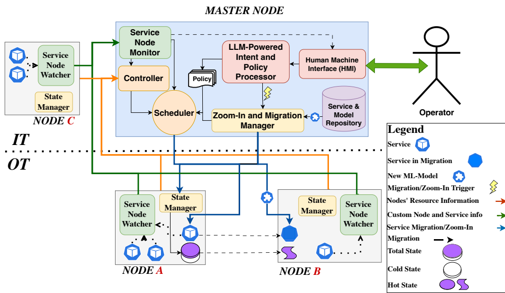
Collective Intelligence-based Service Migration Framework Architecture
