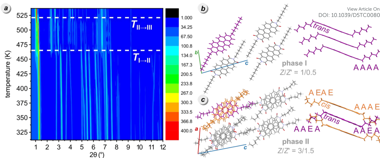
Figure 3. Temperature-resolved powder X-ray diffractograms of PDI-C 6 upon heating (left). The dashed lines indicate the transition temperatures identified in the DSC measurement: T_{I \rightarrow II} = 465 K and T_{II \rightarrow III} = 521 K. The color scale represents intensity variations. Crystal structures of PDI-C 6 phase I (b) and II (c) showing: the packing arrangement along the 1D columnar alignment (left) and the columnar stacking, including conformer descriptors (right). Molecules located at the inversion center with a trans conformation are depicted in purple, while those in general positions with a cis conformation are shown in orange.
