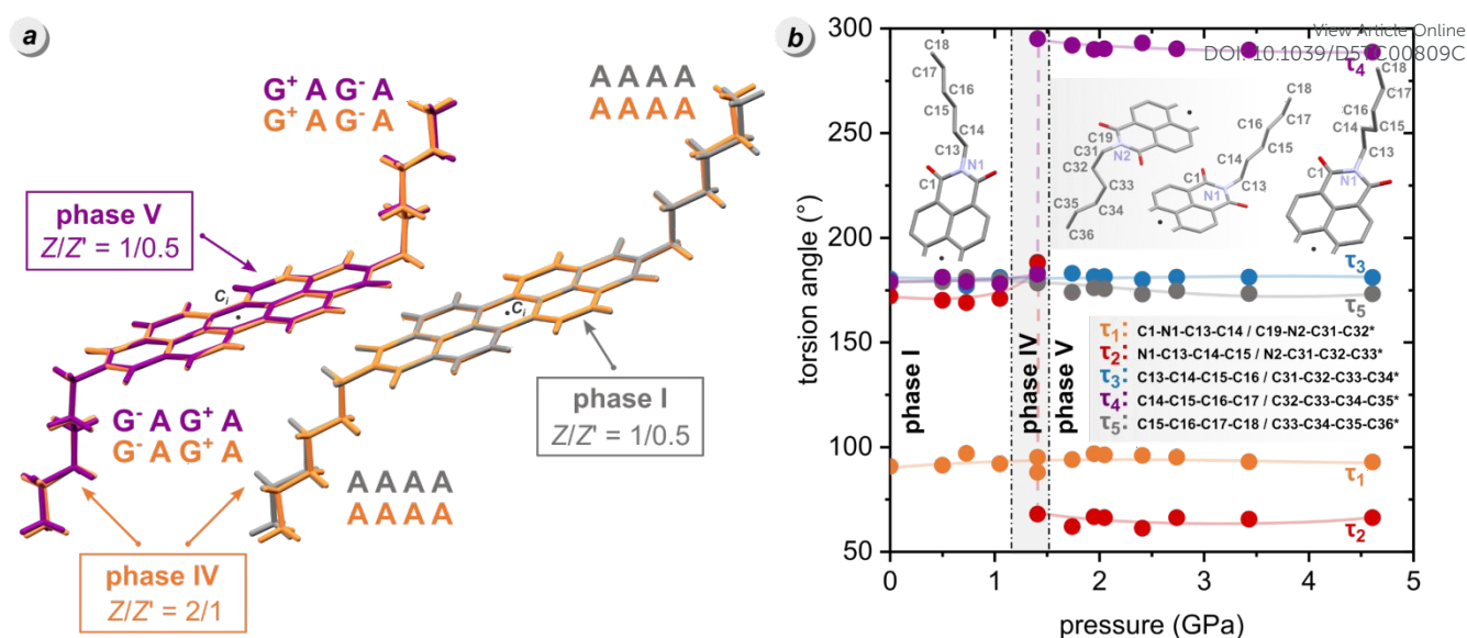
Figure 7. Conformational changes in PDI-C 6 molecules in phases I (grey), IV (orange) and V (violet) illustrated by (a) superimposing fragment of the perylene core, and (b) torsion angles \tau_{1-5} plotted as a function of pressure. In the description of the torsion angles, asterisks refer to the atoms in phase IV. Hydrogen atoms are omitted for clarity.
