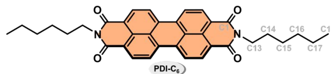
Scheme 1. Structural formula of N,N' -dihexyl-3,4,9,10-perylenedicarboximide (PDI-C 6 ). View Article Online DOI: 10.1039/D5TC00809C
