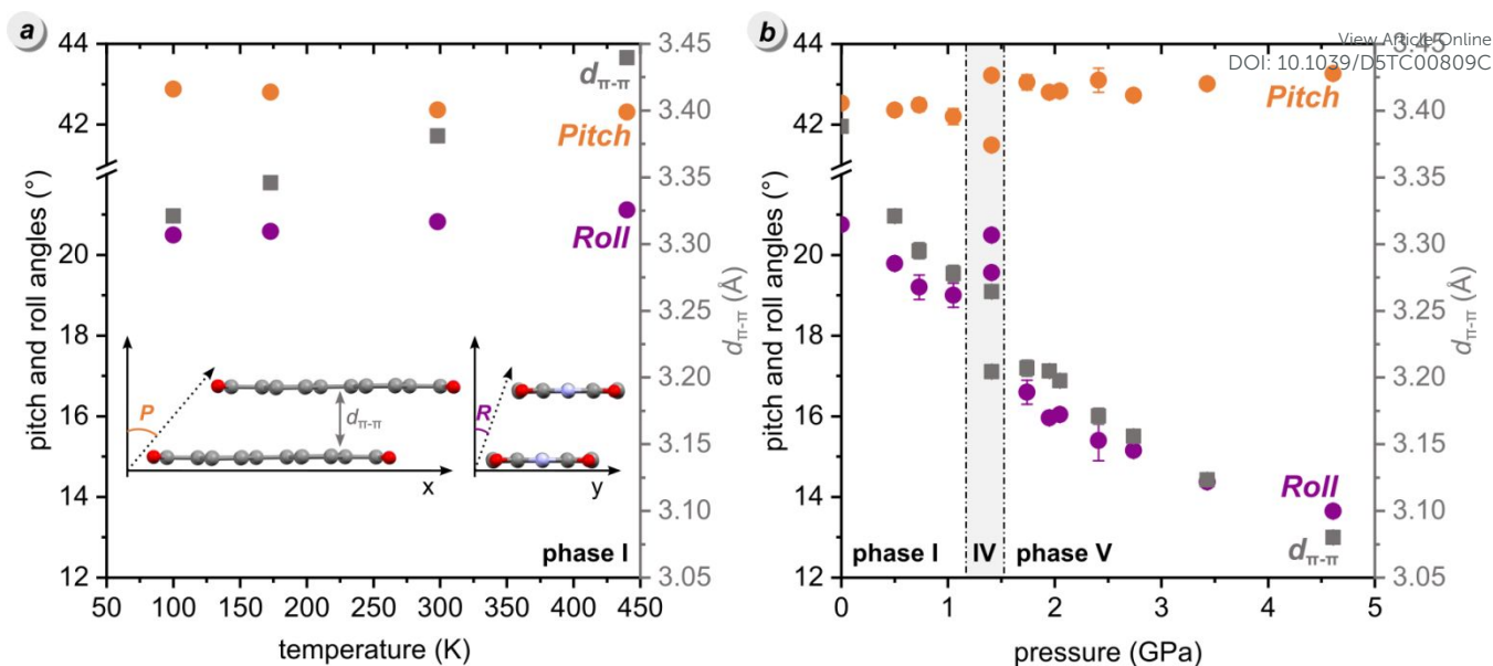
Figure 5. Temperature (a) and pressure (b) effects on the \pi -stacking of PDI-C 6 molecules under pressure: orange and purple symbols represent the pitch and roll angles and grey squares mark the distance between \pi -stacked molecules ( d_{\pi-\pi} ). 61 Inset: graphical representation of P , R and d_{\pi-\pi} . The alkyl substituents and H-atoms are skipped for clarity. The corresponding numerical values can be found in Tables S2 and S10 of the SI.
