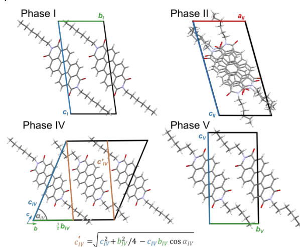
Figure 6. Lattice relations between phases I (0.1 MPa/298 K), II (0.1 MPa/470 K), IV (1.41 GPa/296 K), and V (1.95 GPa/296 K) in PDI-C 6 , illustrated for maintained orientations of the \pi -stacked molecules; the orange axes in phase IV indicate the corresponding directions in phases I and V.
