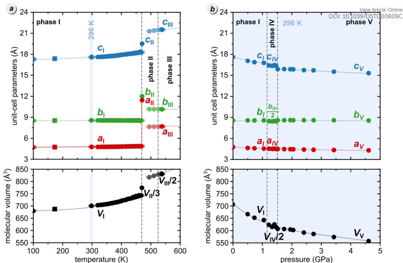
Figure 4. Temperature (a) and pressure (b) dependence of the unit-cell dimensions a , b , c (top) and molecular volume ( V_m = V/Z , bottom) of PDI- C_6 . Estimated standard deviations (ESDs) are smaller than plotted symbols. The data at 173 K (squares) were taken from Madhu et al. 45 The unit-cell parameters of phase III determined during the cooling cycle are marked with a lighter color. The data measured at 296 K is highlighted in blue. Lines joining the points are for guiding the eye only. The triclinic angles are plotted in Figure S21.
