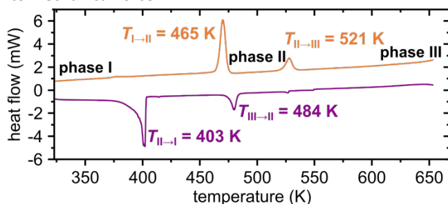
Figure 1. Differential scanning calorimetry (DSC) thermogram of PDI-C 6 in the heating (top) and cooling (bottom) cycles. Temperatures of phase transitions are indicated.
