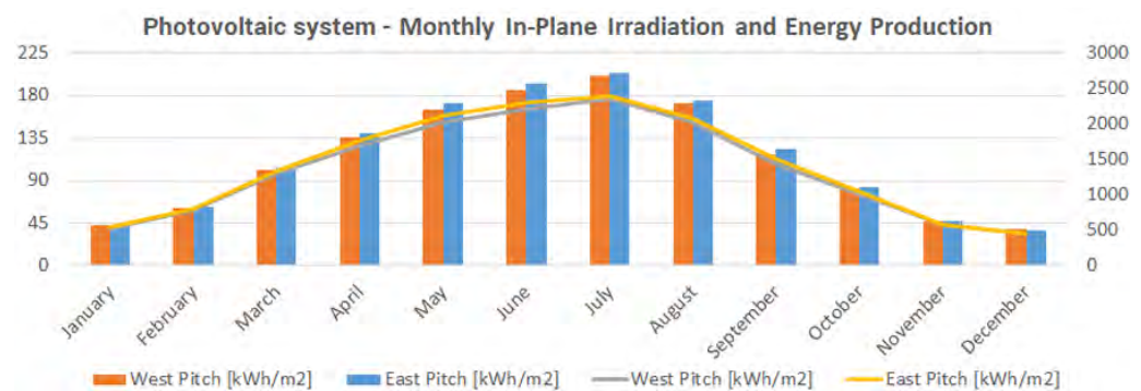
Figure 9. Monthly energy output from fixed-angle PV systems and monthly in-plane irradiation evaluated for the retrofit scenario (RIQ)—© Authors.
