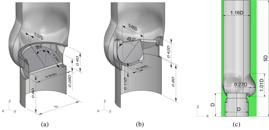
Figure 1: Cutaway view of three-dimensional model of the aortic root-housing-leaflets assembly with the principal measurements: (a) bileaflet mechanical valve, (b) trileaflet mechanical valve. (c) Front view of the valve-aortic root arrangement immersed in the computational domain (green area).
