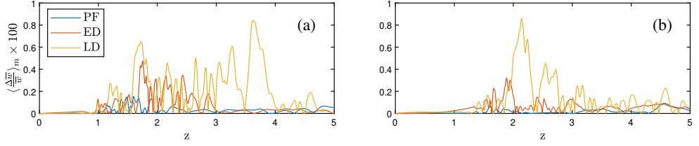
Figure 28: Streamwise distribution of relative monitor line-averaged variation in the streamwise velocity component from the 17 th to the 18 th cycle
