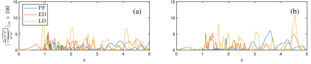
Figure 30: Streamwise distribution of relative monitor line-averaged variation in the isotropic streamwise Reynolds stress component from the 17 th to the 18 th cycle
