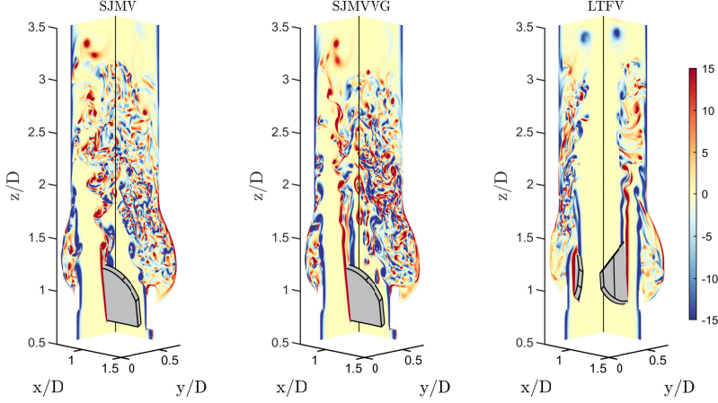
Figure 8: Contours of instantaneous out-of-plane vorticity ( \omega_x D/U and \omega_y D/U ) over the longitudinal cross-sections of the aortic root in the ED stage.
