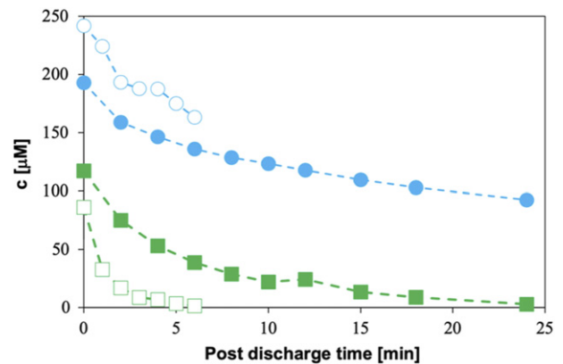
Figure 17. Evolution of the concentration of reactive species in DIW after air plasma treatments of 5 or 10 min (filled and empty symbols, respectively); green squares refer to H 2 O 2 and blue circles to NO 2 - , the conjugate base of nitrous acid. Reprinted from [74], Copyright (2015), with permission from Elsevier.
