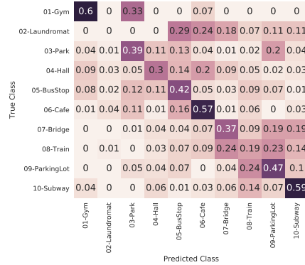
Fig. 4: Confusion Matrix for the best configuration: Leave-a-Place-Out.
