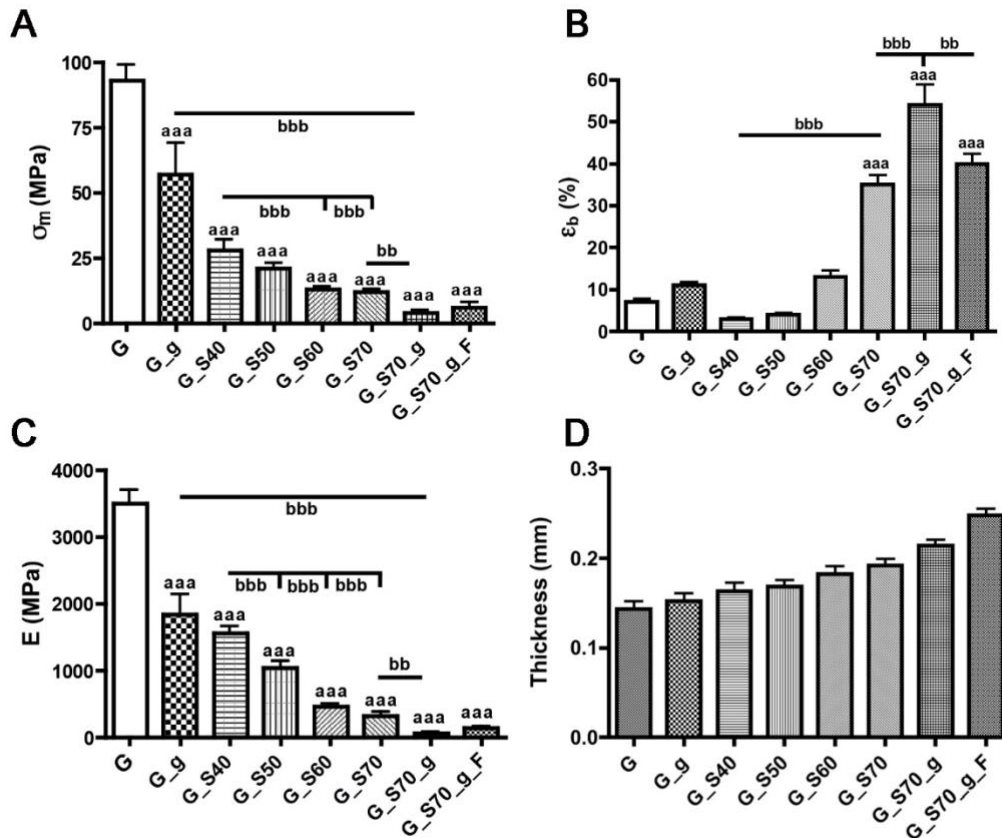
Figure 7: A-C: Mechanical properties of gelatin-based films: A) maximum stress at break ( \sigma_m , aaa p < 0,001 compared to G; bbb p < 0,001 G_g vs G_S70_g, G_S40 vs G_S60 and G_S40 vs G_S70); B) elongation % at break ( \epsilon_b ; aaa p < 0,001 compared to G; bbb p < 0,001 G_S40 vs G_S70, G_S70 vs G_S70_g and bb p < 0,01 G_S70_g vs G_S70_g_F); C) Elastic modulus (E, aaa p < 0,001 compared to G; bbb p < 0,001 G_g vs G_S70_g, G_S40 vs G_S50, G_S40 vs G_S60 and G_S40 vs G_S70); D) Thicknesses of gelatin-based films.
