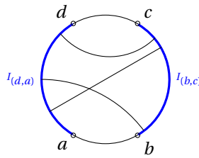
Figure 1. The rectangle R \subseteq \partial\mathcal{H}^2 \times \partial\mathcal{H}^2
