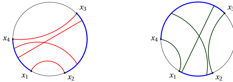
Figure 3. On the left the rectangle associated to CR(\ell_1, \ell_2, \ell_3, \ell_4) , and on the right the one associated to CR(\ell_4, \ell_1, \ell_2, \ell_3) .
